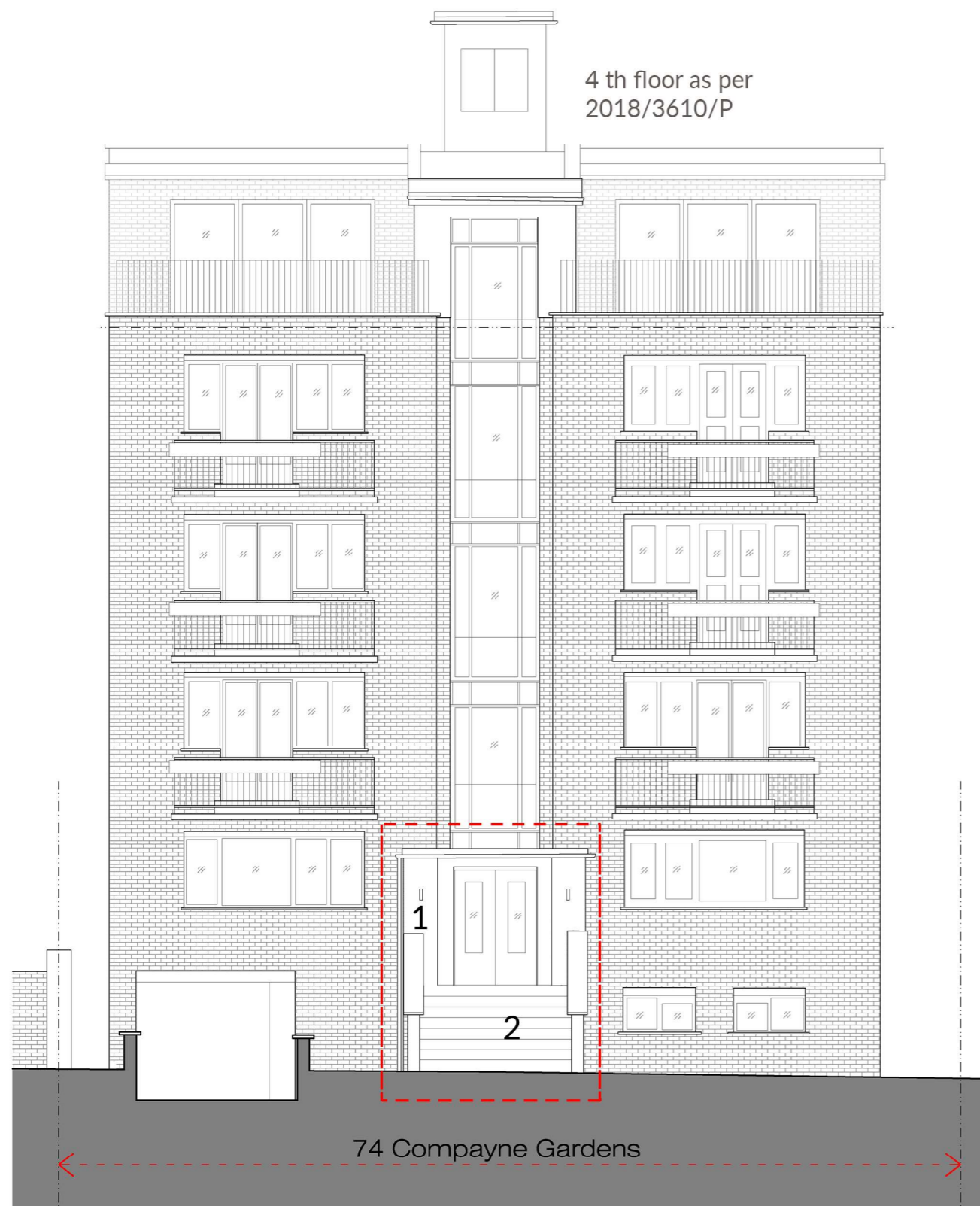
Proposed Front Elevation Scale 1:100
