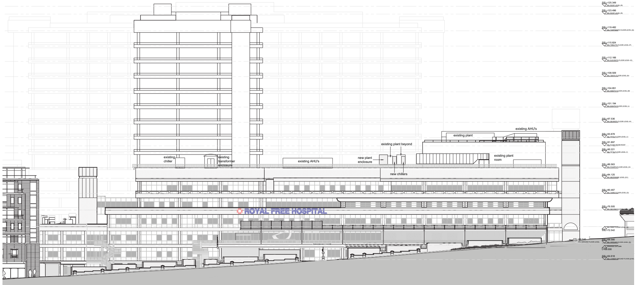
NORTH ELEVATION
