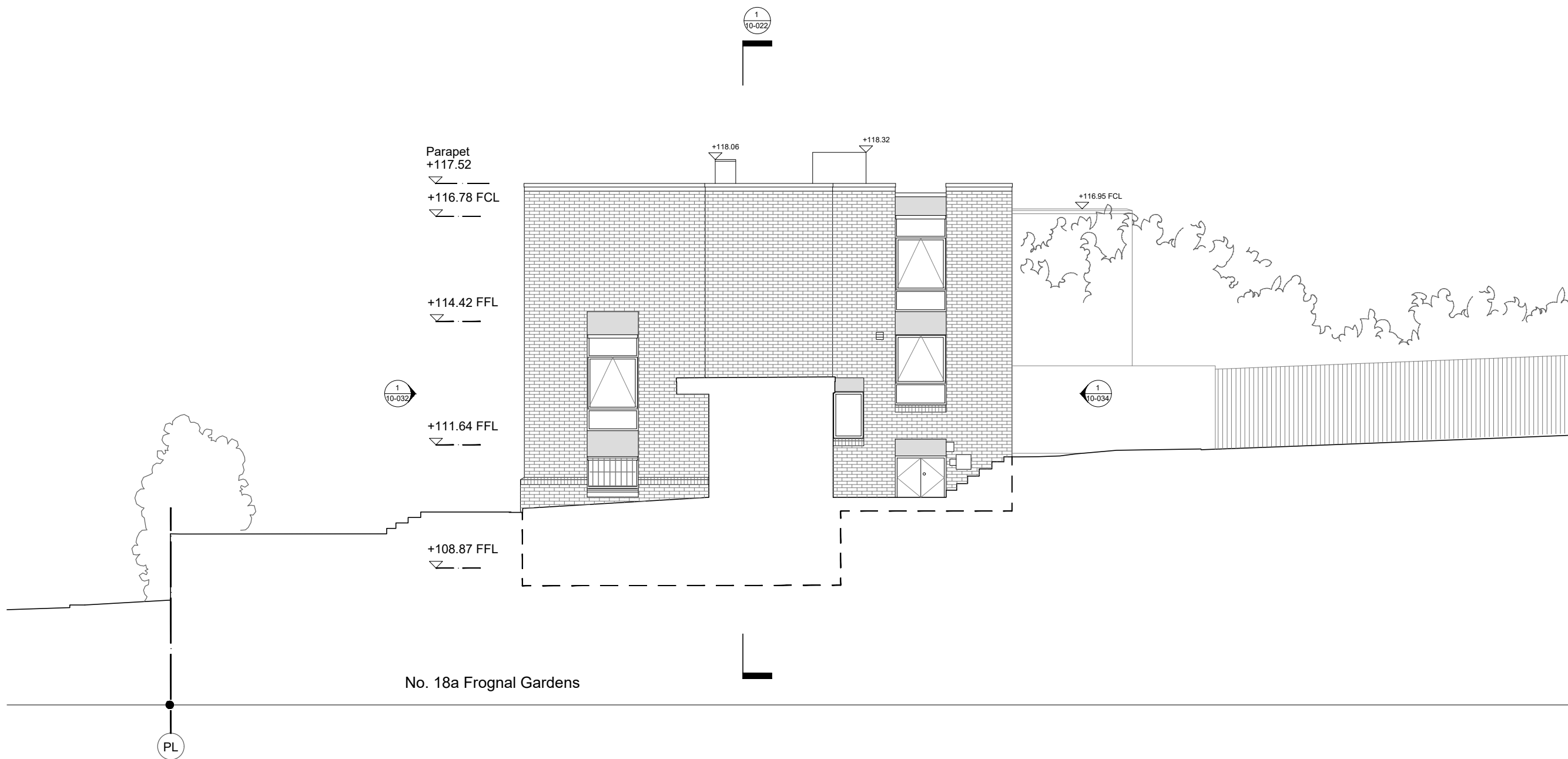
1 EXISTING SOUTH ELEVATION
