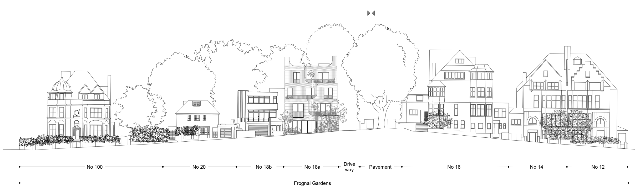
1 Unfolded Street Elevation SCALE 0 10 m
