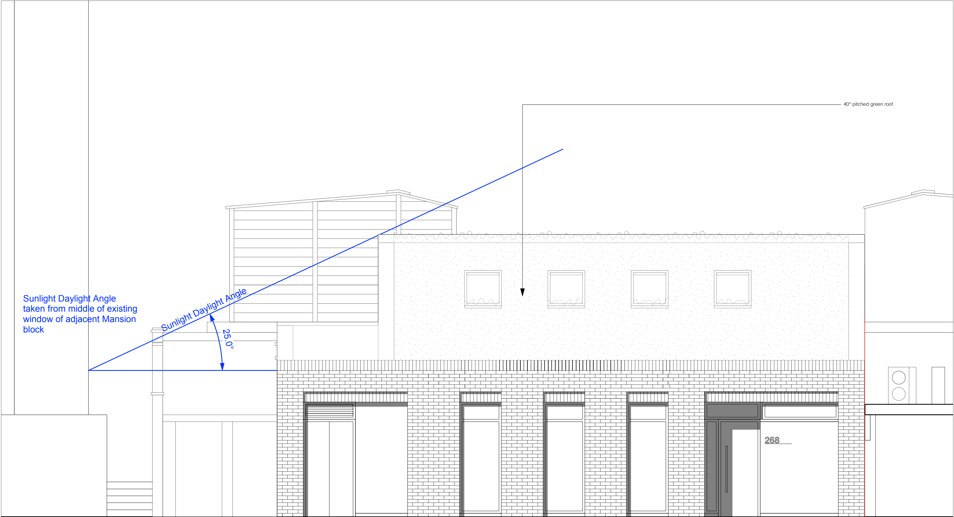
Proposed Section Elevation AA
