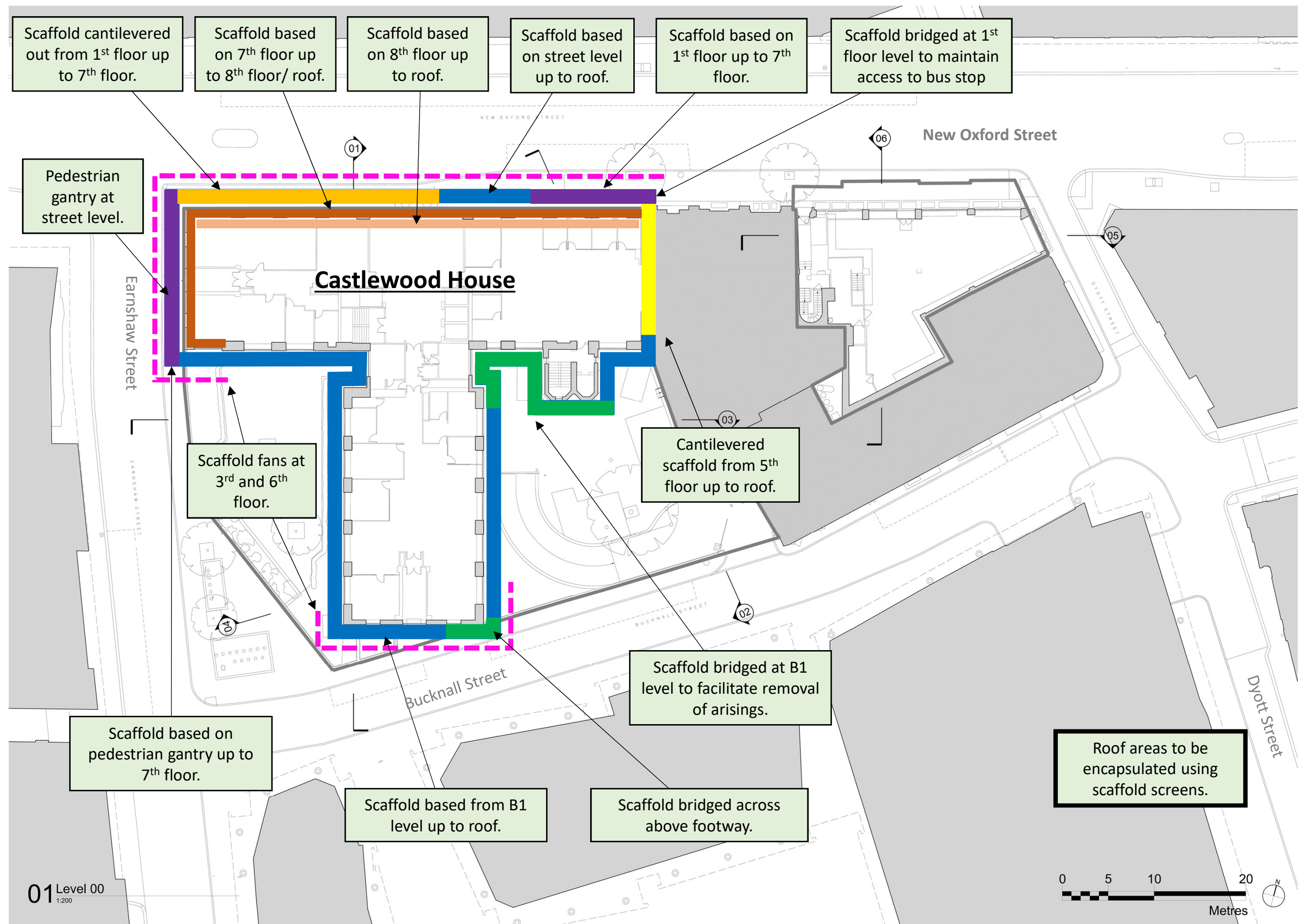
Castlewood House Scaffold Plan
