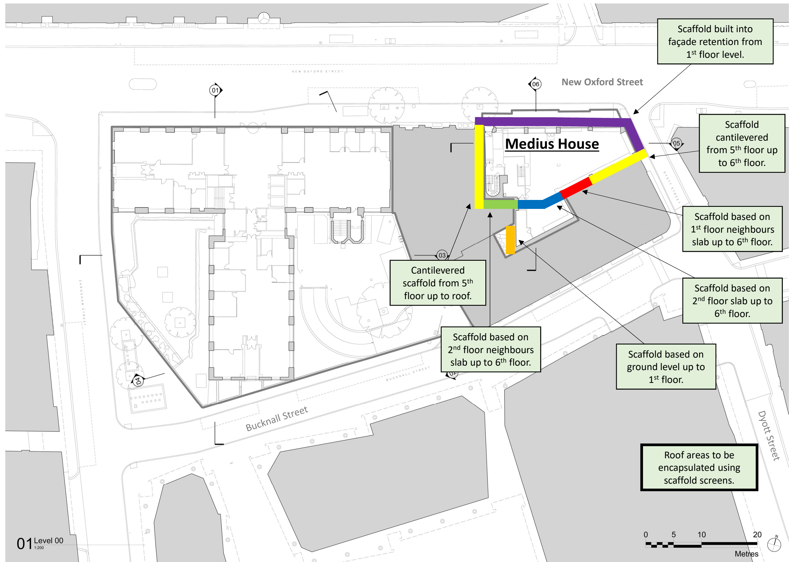
Medius House Scaffold Plan
