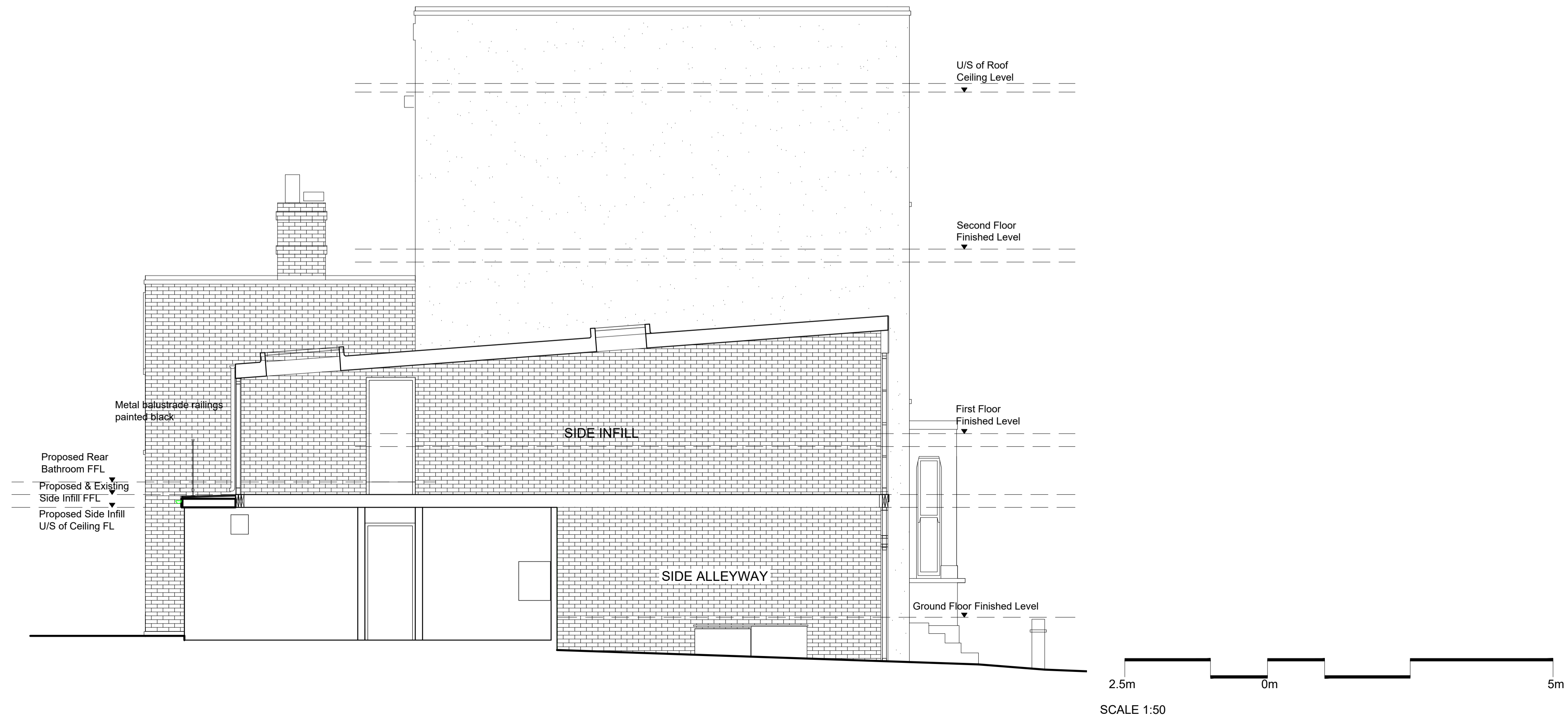
02:PROPOSED SIDE ELEVATION B SCALE 1:50
