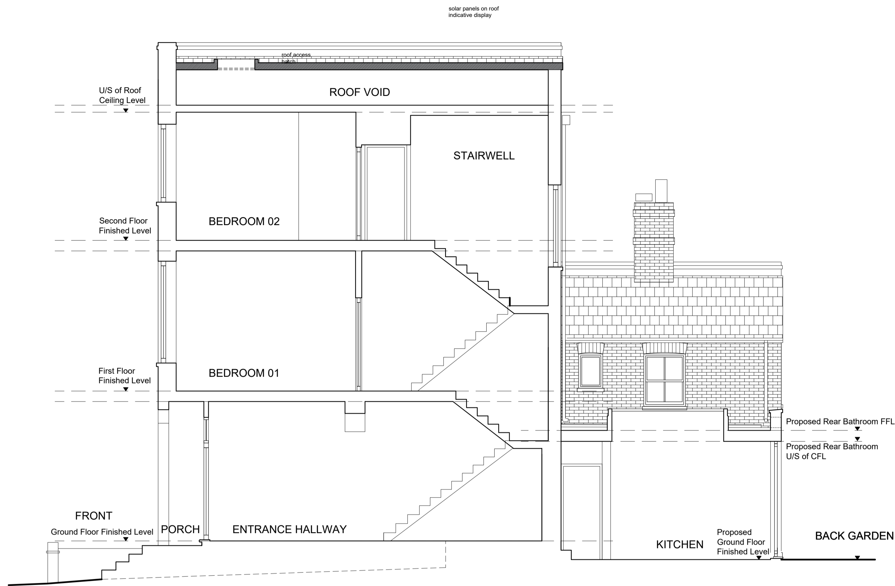
01:PROPOSED SIDE ELEVATION A SCALE 1:50
