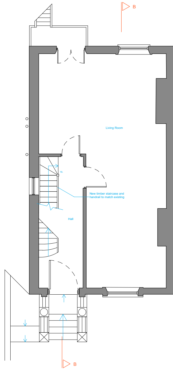
2 Ground Floor Plan
