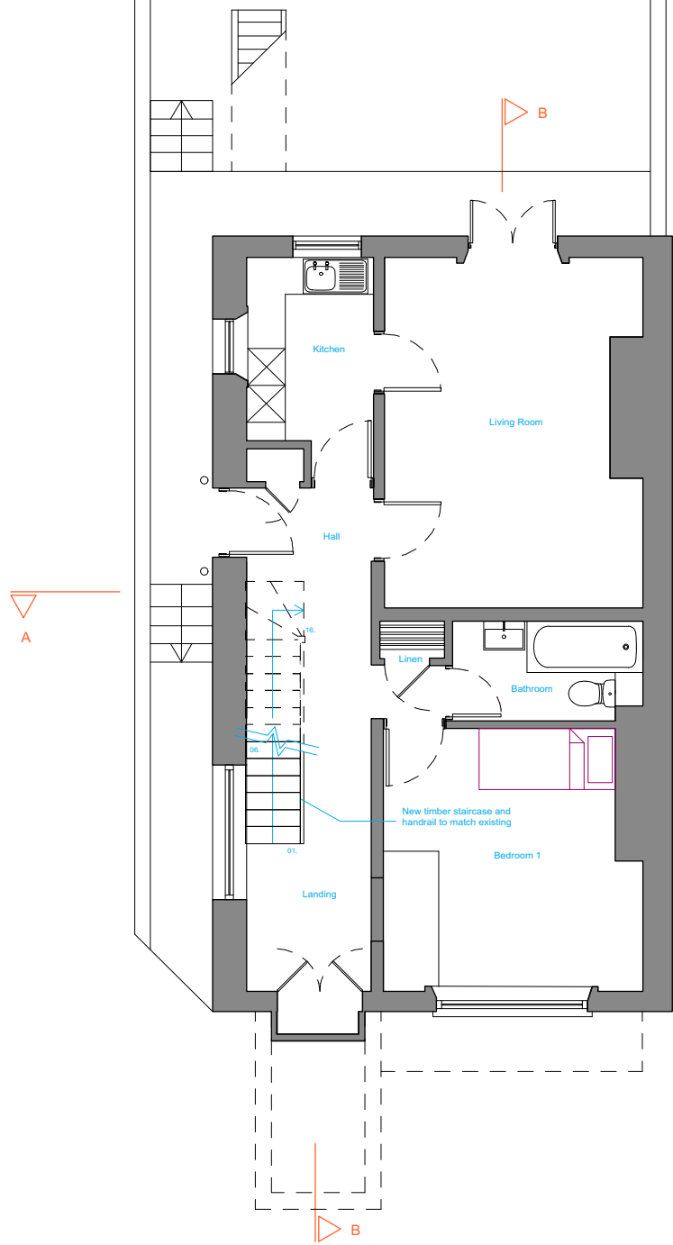
1 Lower Ground Floor Plan
