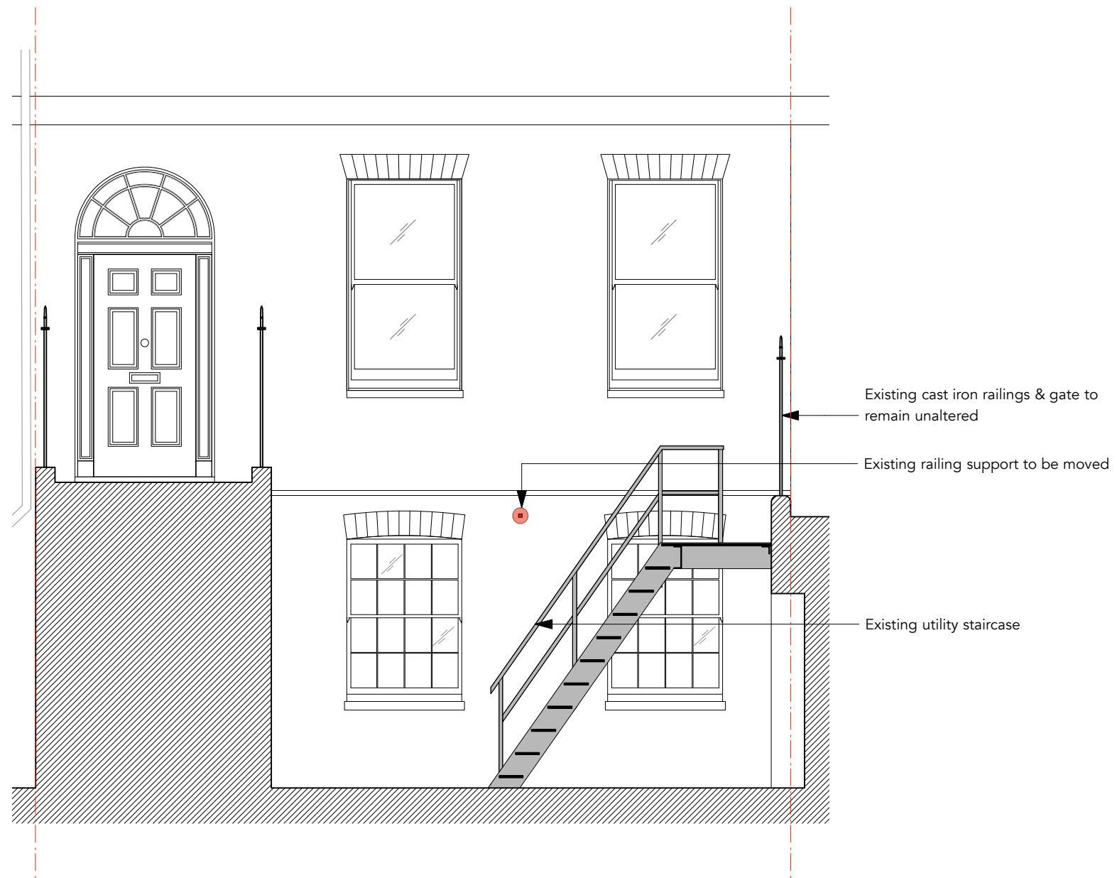
6 Existing Section C-C 1:50
