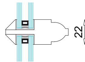
Vertical section of the glazing bar SCALE 1:2
