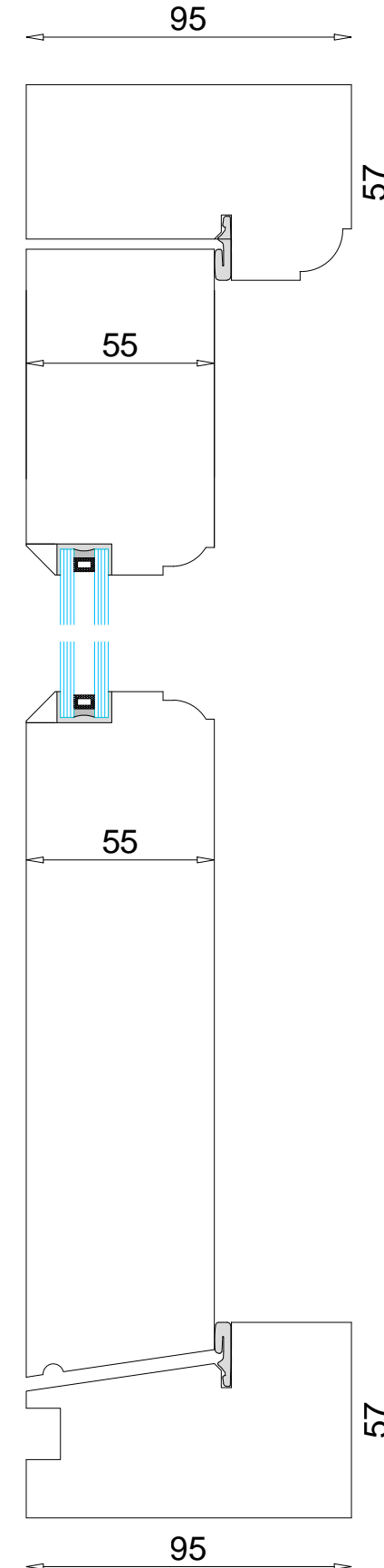
Vertical section SCALE 1:2
