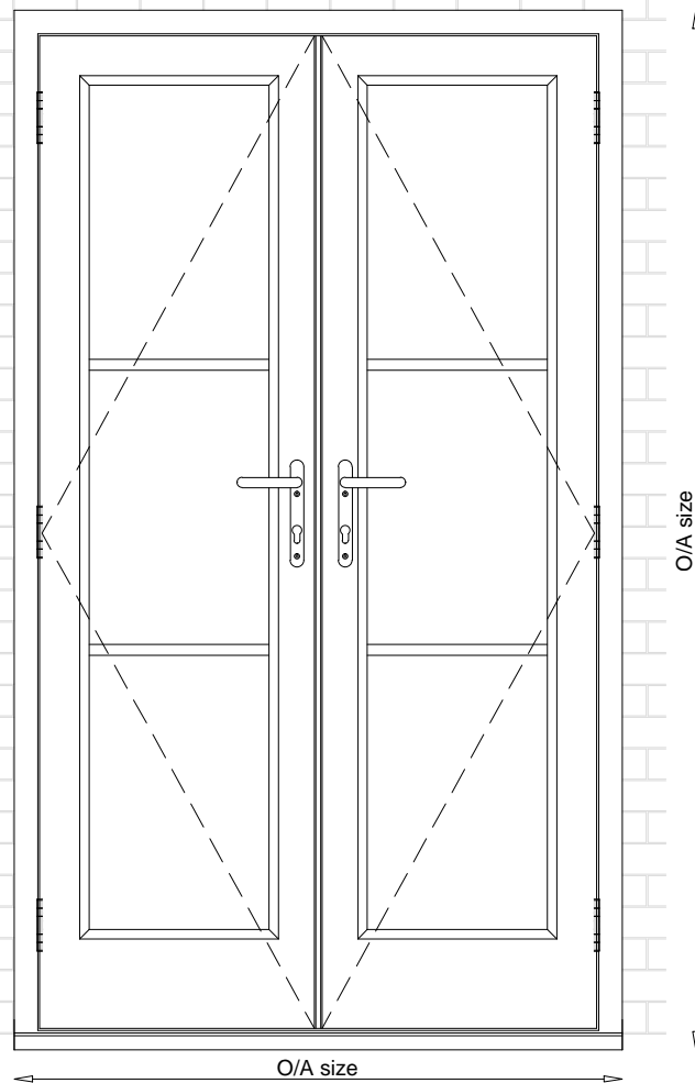
Elevation view from outside
