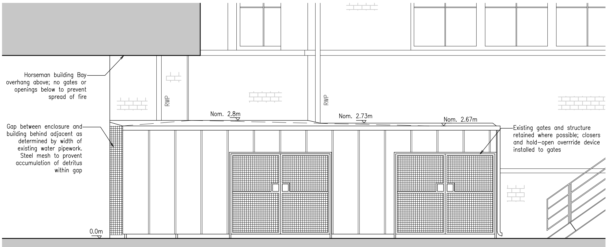
01 Proposed Elevation A SCALE 1:50
