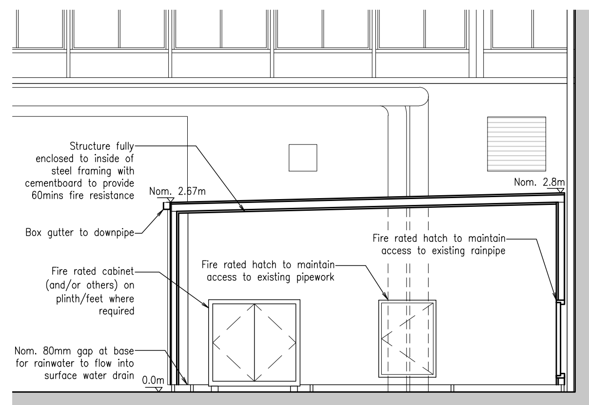
03 Proposed Section X SCALE 1:50
