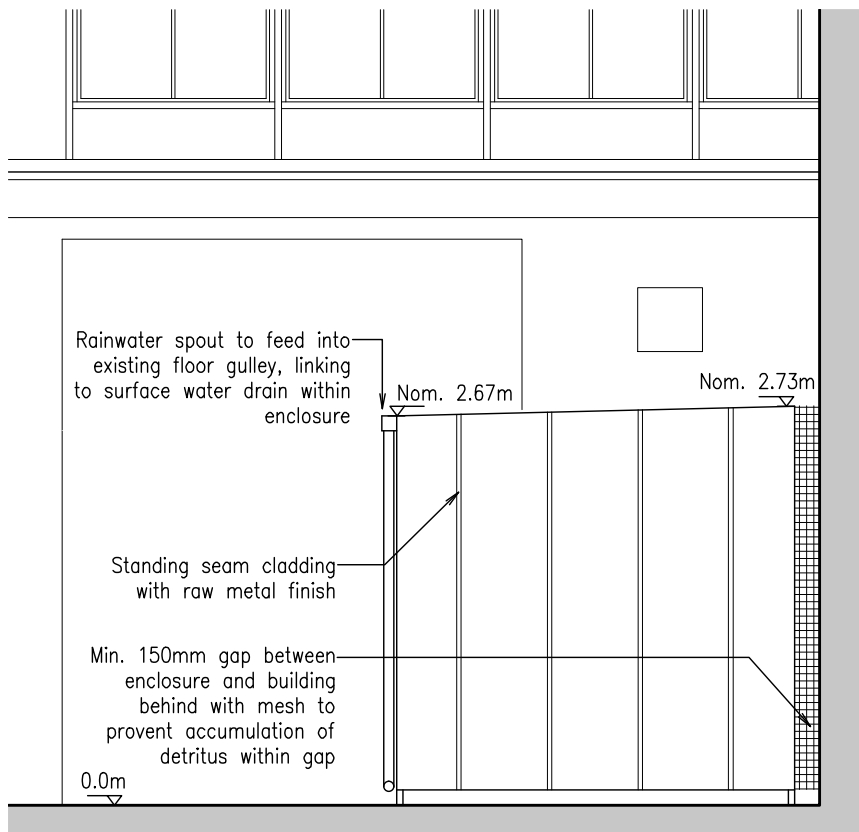
02 Proposed Elevation B SCALE 1:50
