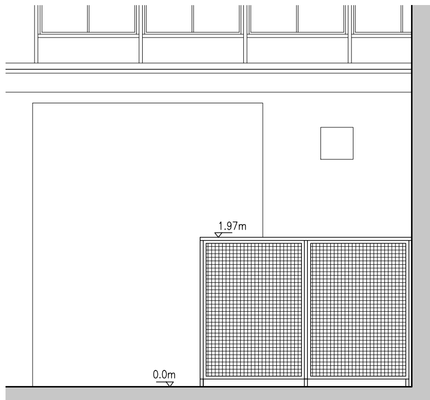
02 Existing Elevation B SCALE 1:50
