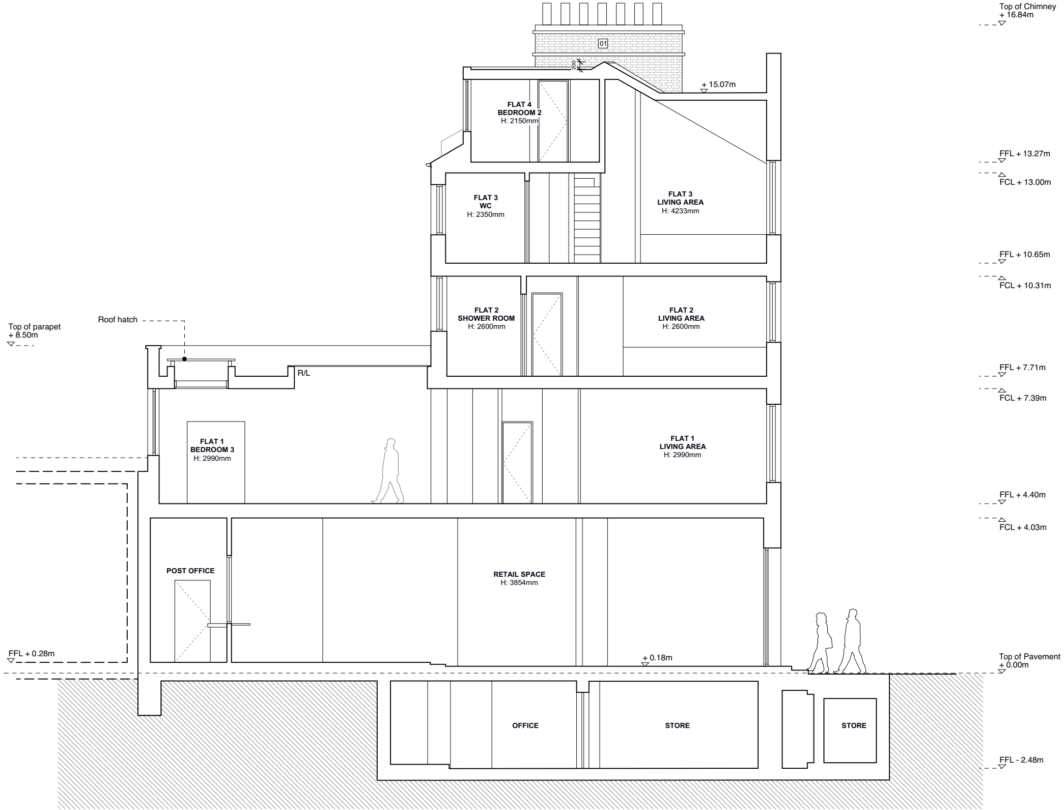
SECTION AA AS PROPOSED - REV E Scale: 1:100 @ A3
