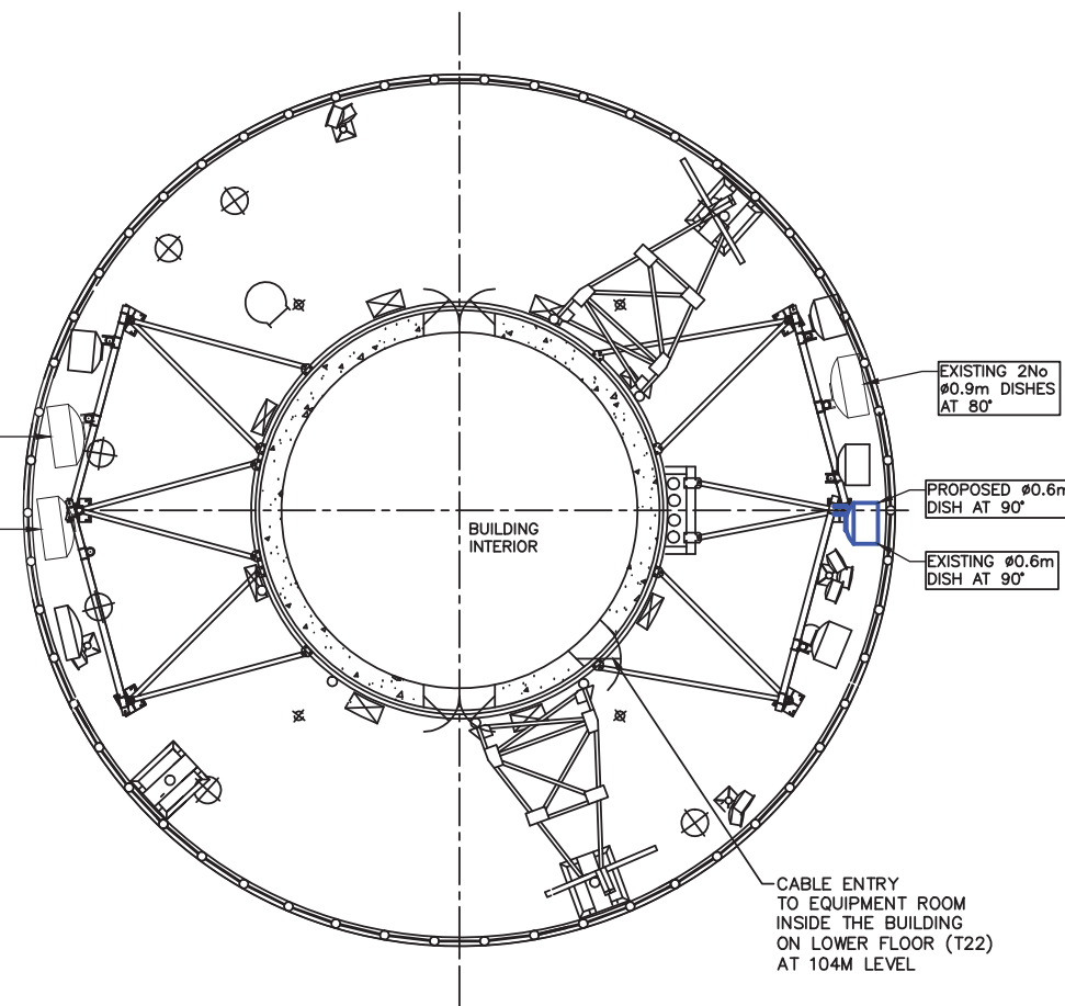
PLAN VIEW ON 133.960m LEVEL SHOWING PROPOSED LAYOUT
