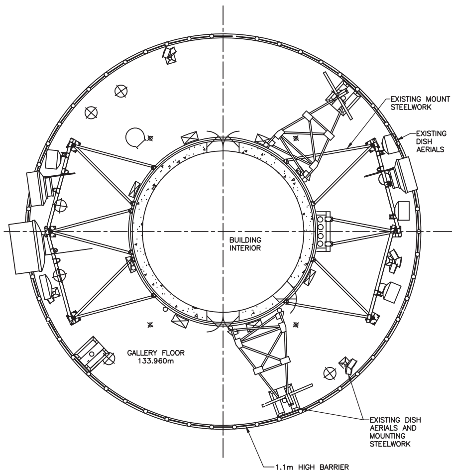
PLAN VIEW ON 133.960m LEVEL SHOWING EXISTING LAYOUT
