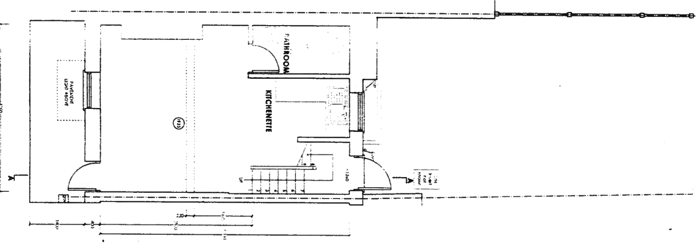
BASEMENT PLAN
