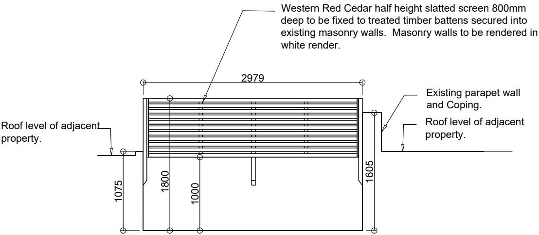
Garden Screening detail Section B-B Scale 1:50
