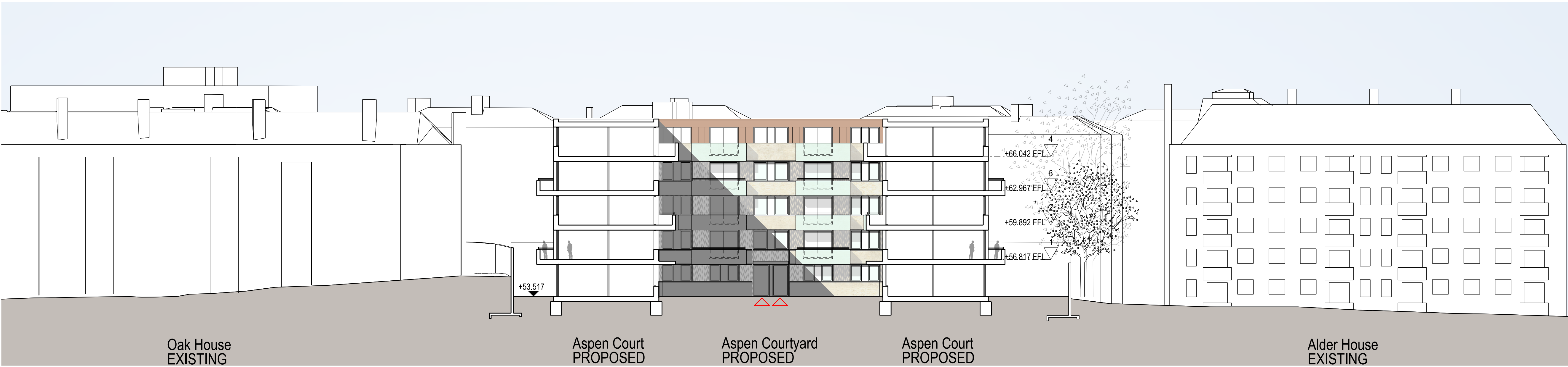
S03 Section 2 Looking West P26 1:200
