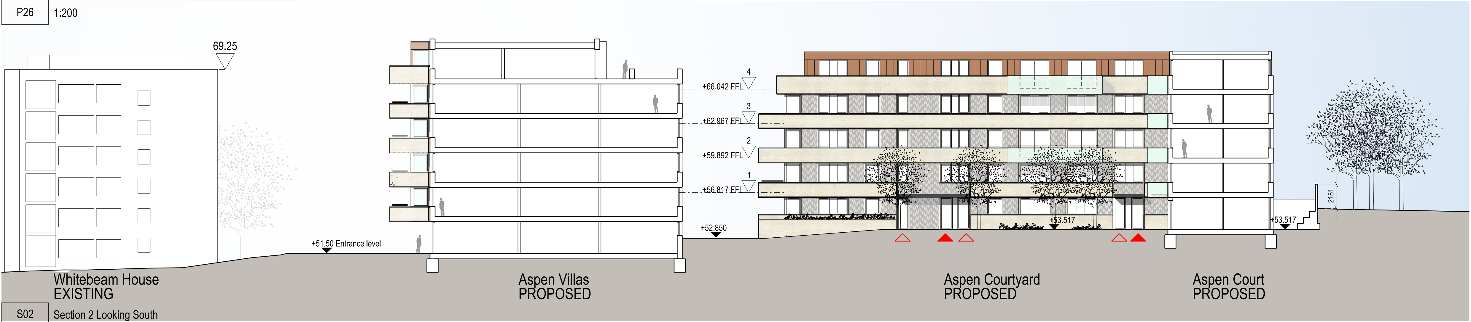
S02 Section 2 Looking South P26 1:200
