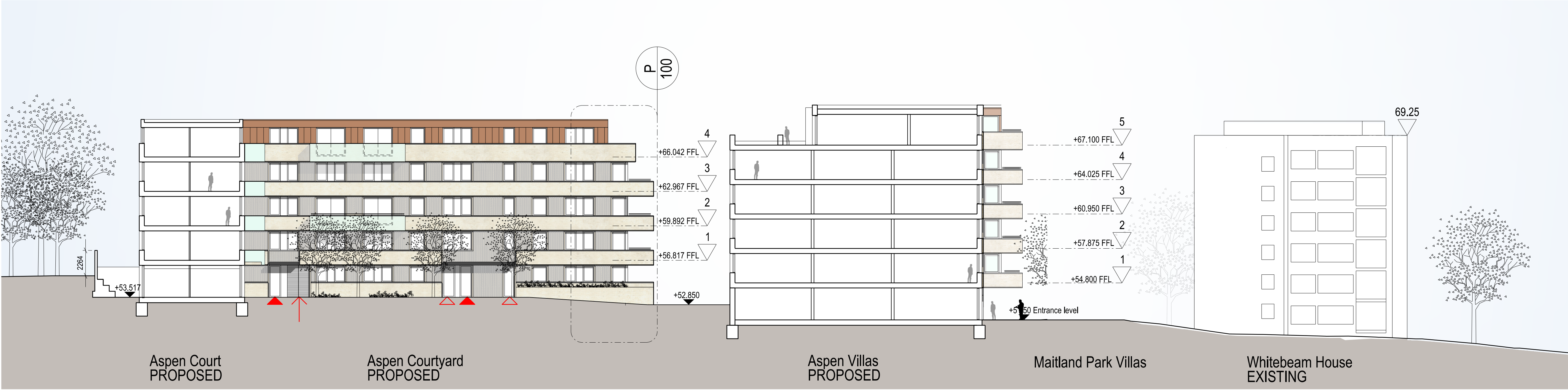
S01 Section 1 Looking North P26 1:200
