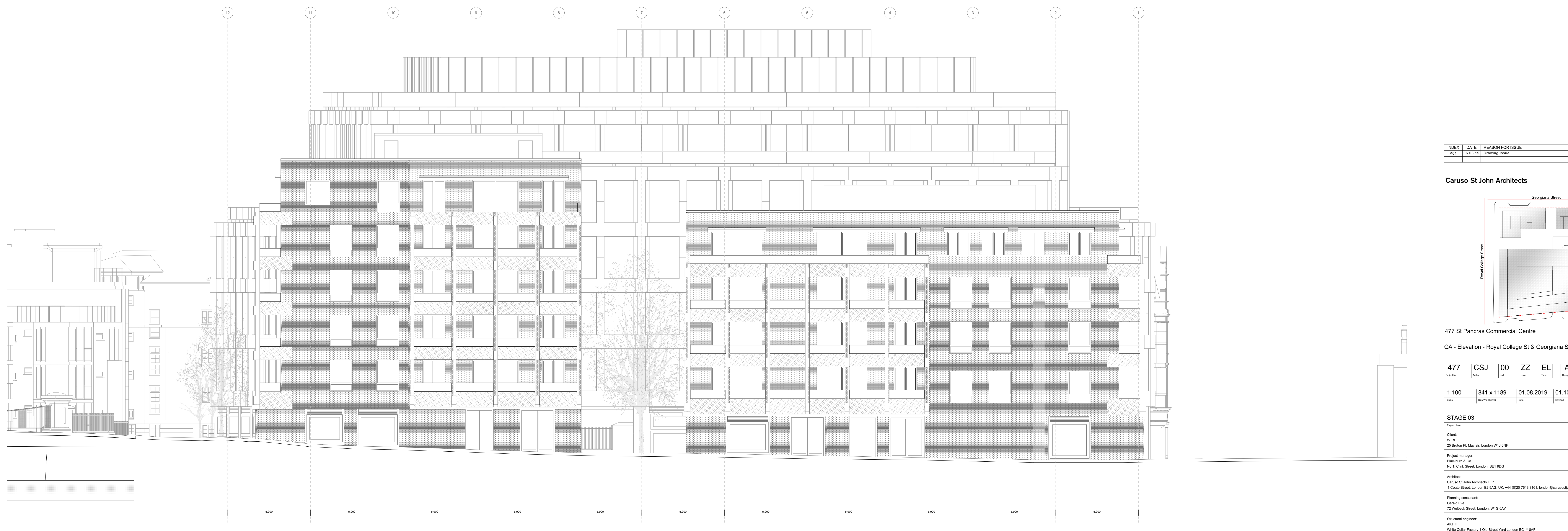
Elevation - Royal College Street
