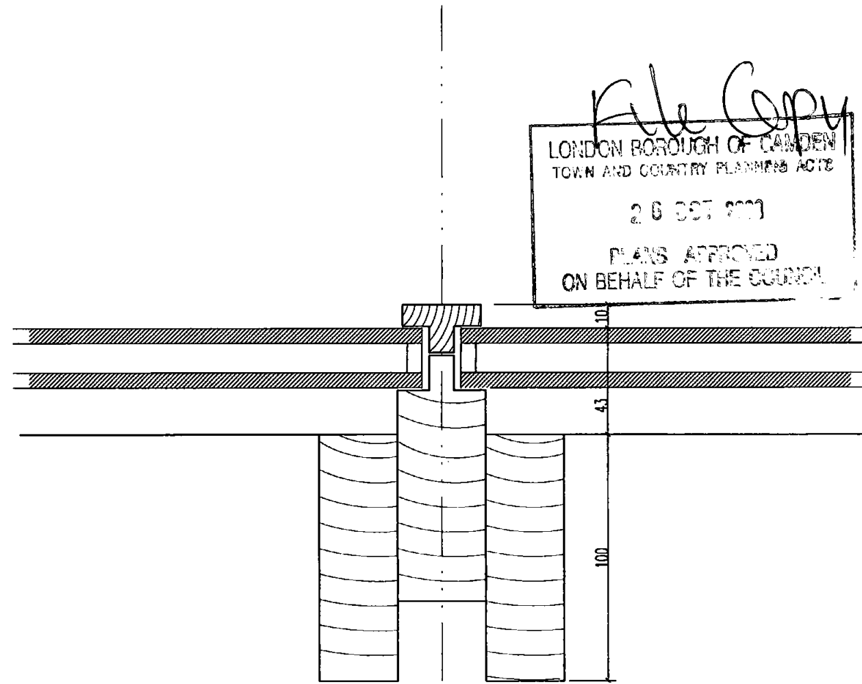
Existing Typical Glazing Section (Mullion)
