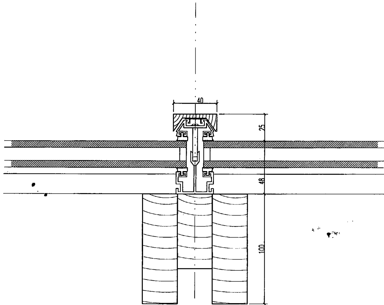
Proposed Typical Glazing Section (Mullion)
