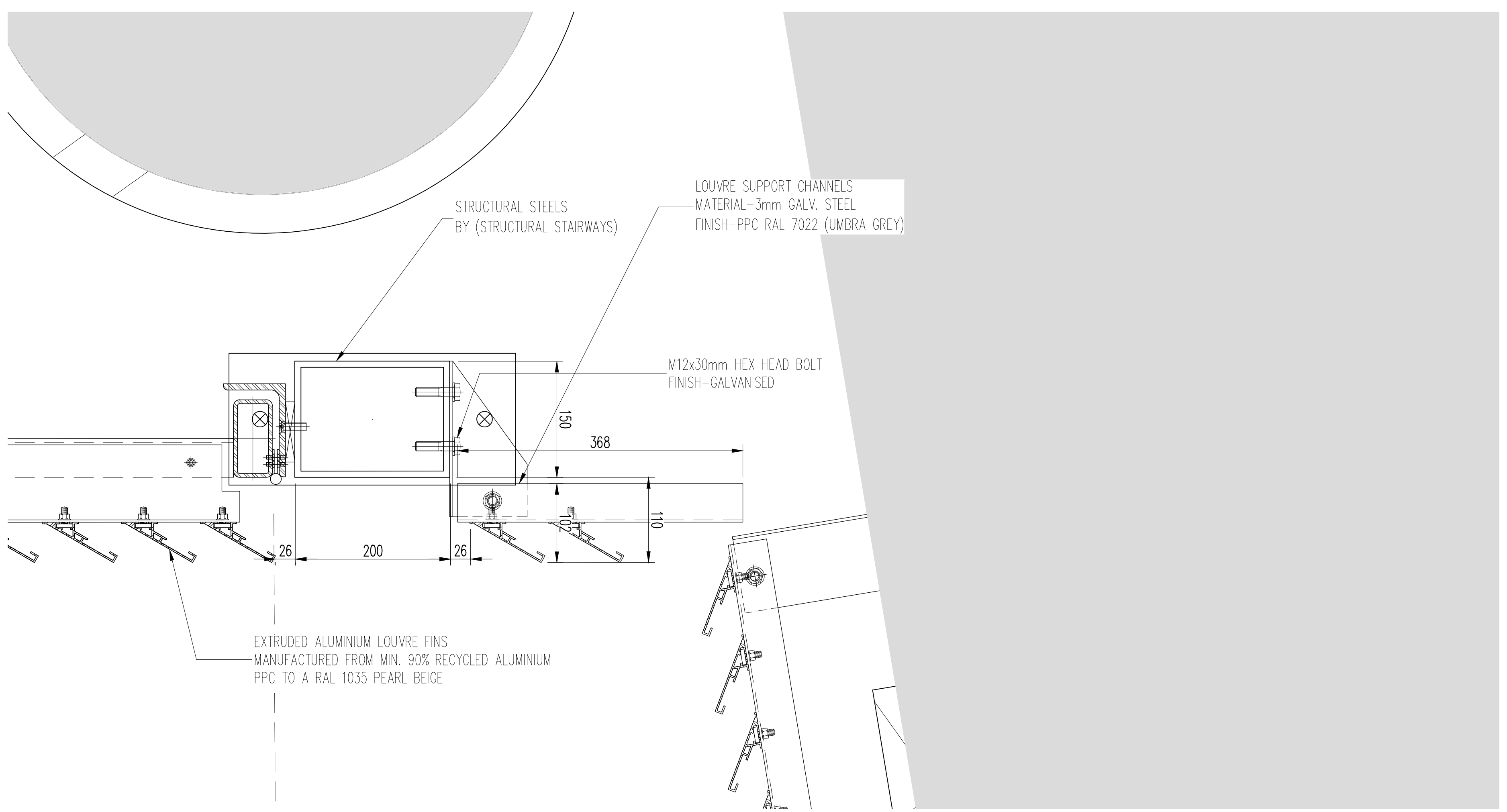
02 HORIZONTAL SECTION 1:4
