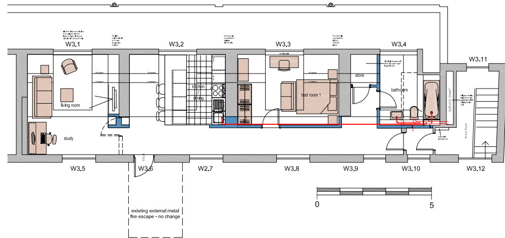
THIRD FLOOR PLAN AS PROPOSED 1:100
