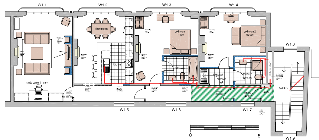
FIRST FLOOR PLAN AS PROPOSED 1:100
