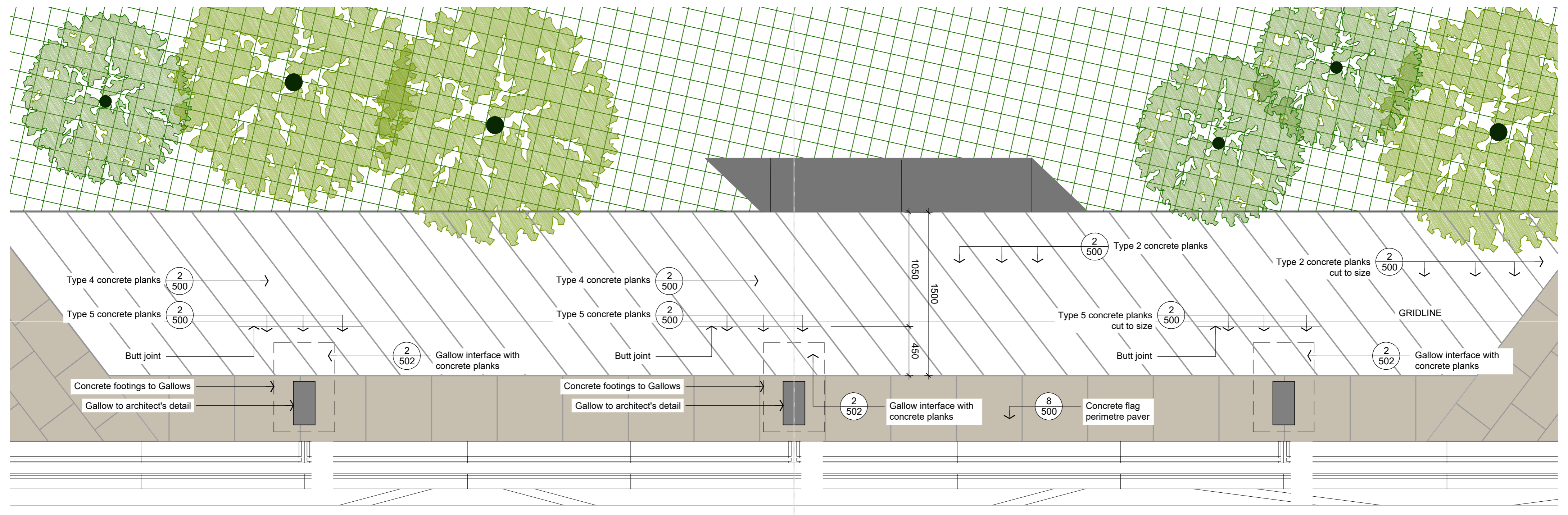
2 CONCRETE PLANKS - S2 TERRACES - LEVEL 8 DETAILED PLAN SCALE 1:25
