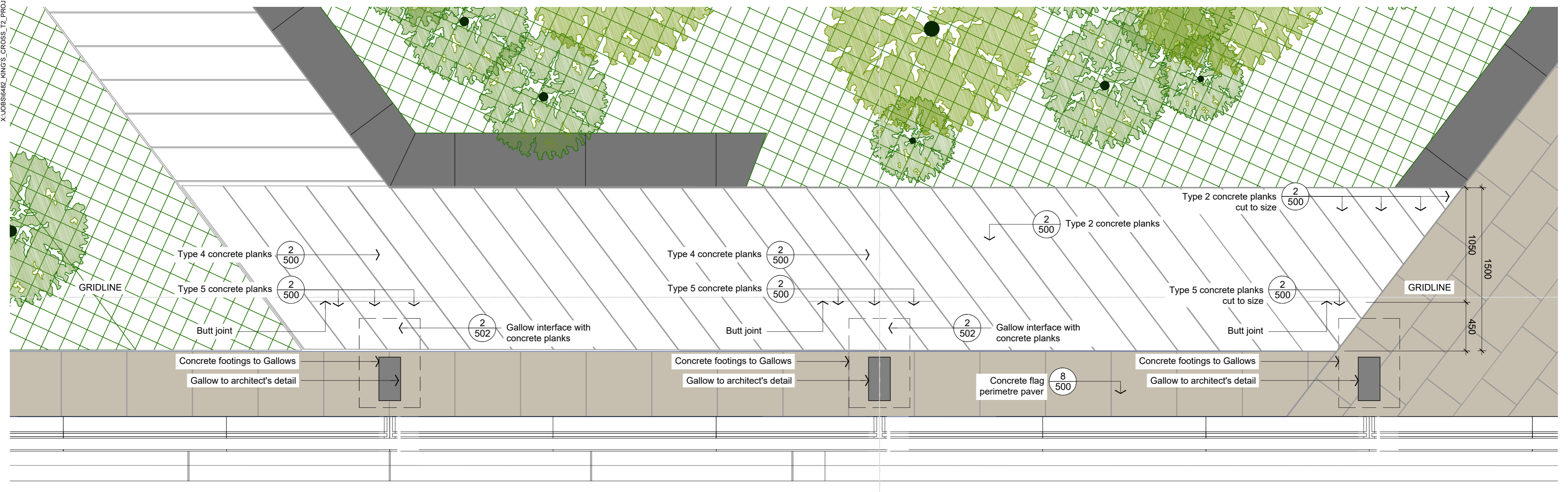
1 CONCRETE PLANKS - S1 TERRACES - LEVEL 8 DETAILED PLAN SCALE 1:25
