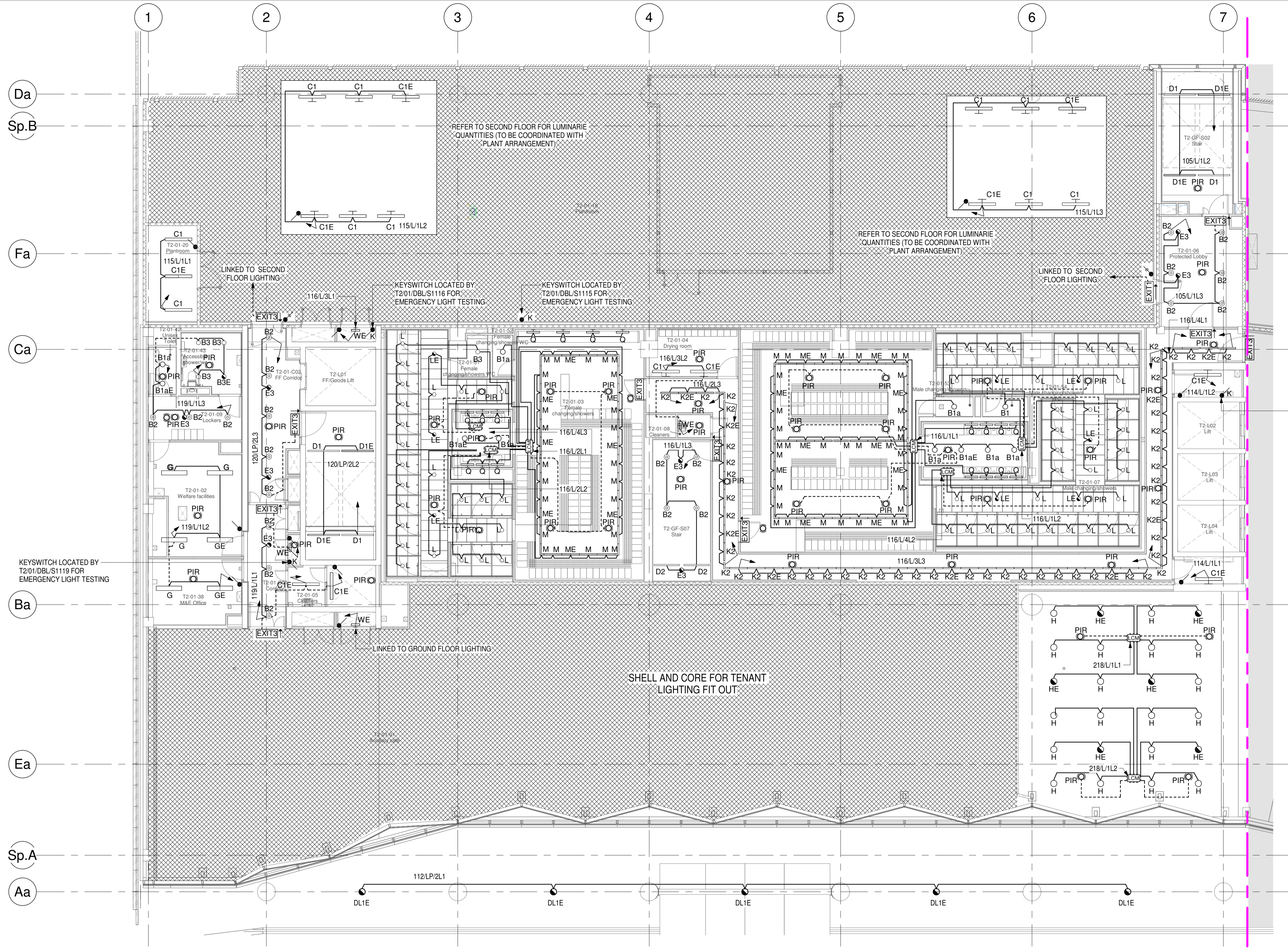
1 Lighting Layout Level 01 (Block S1) 1 : 100
