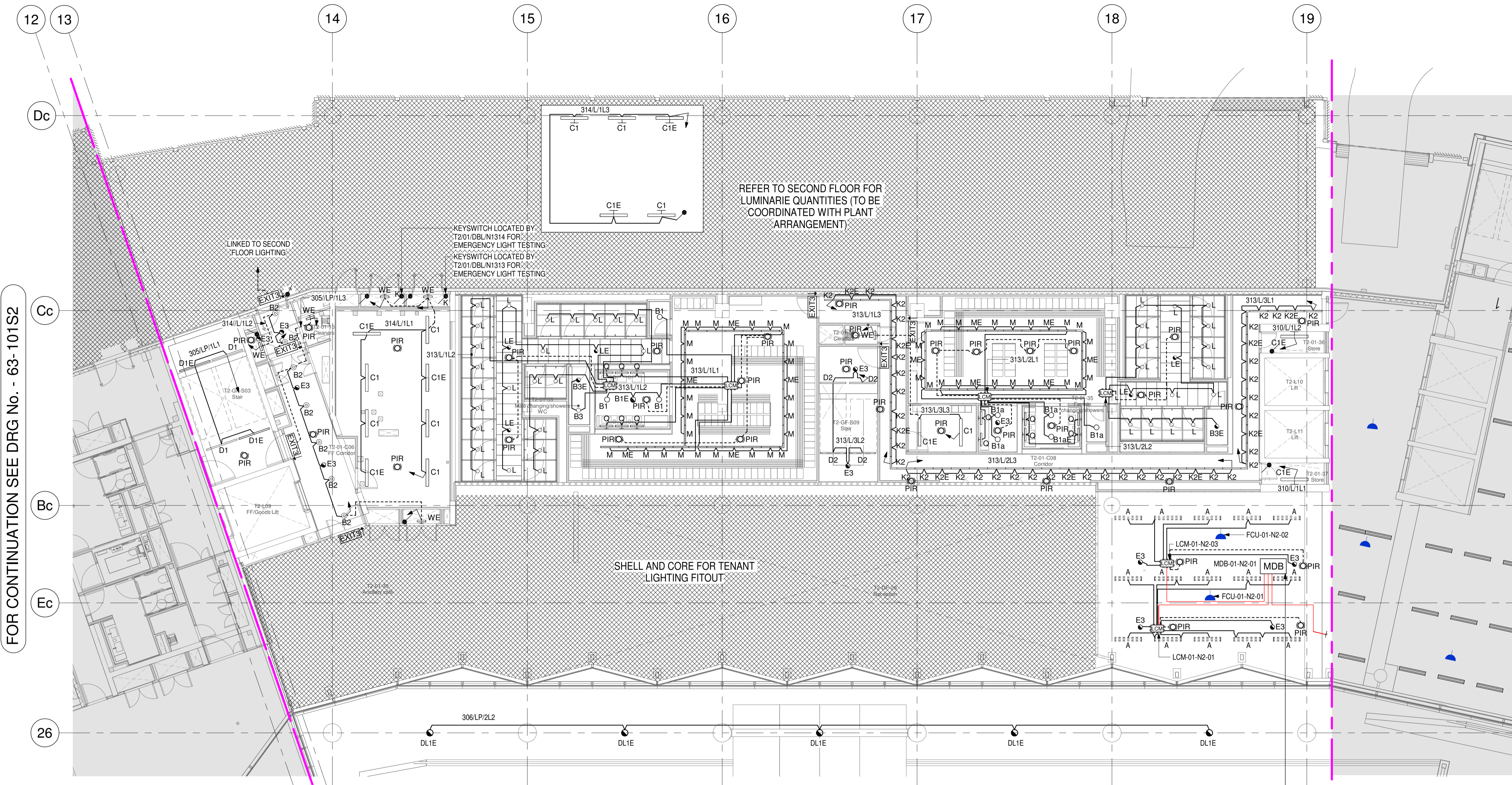
1 Lighting Layout Level 01 (Block N1) 1 : 100
