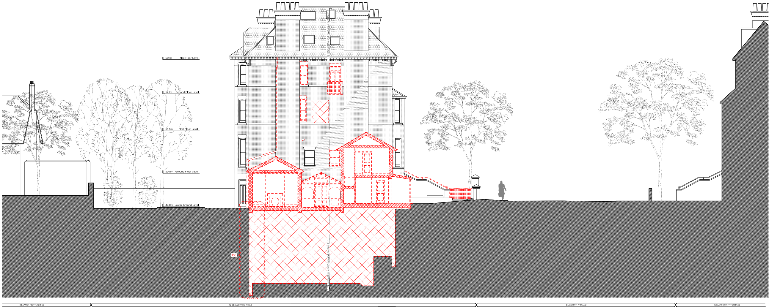
Demolition Section C-C
