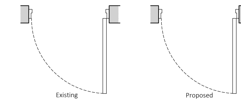
Plan Note: Replace existing 4 panel timber door with new jib door.
