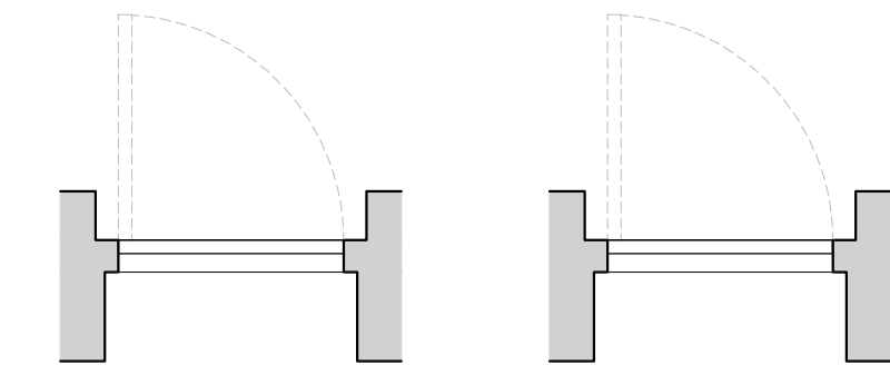
Plan Note: Existing timber 4-panel door to be replaced with single panel timber framed double glazed door.
