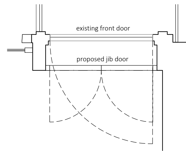
Plan Note: New plain double jib door to inside of existing front door. 54mm thick with acoustic core.
