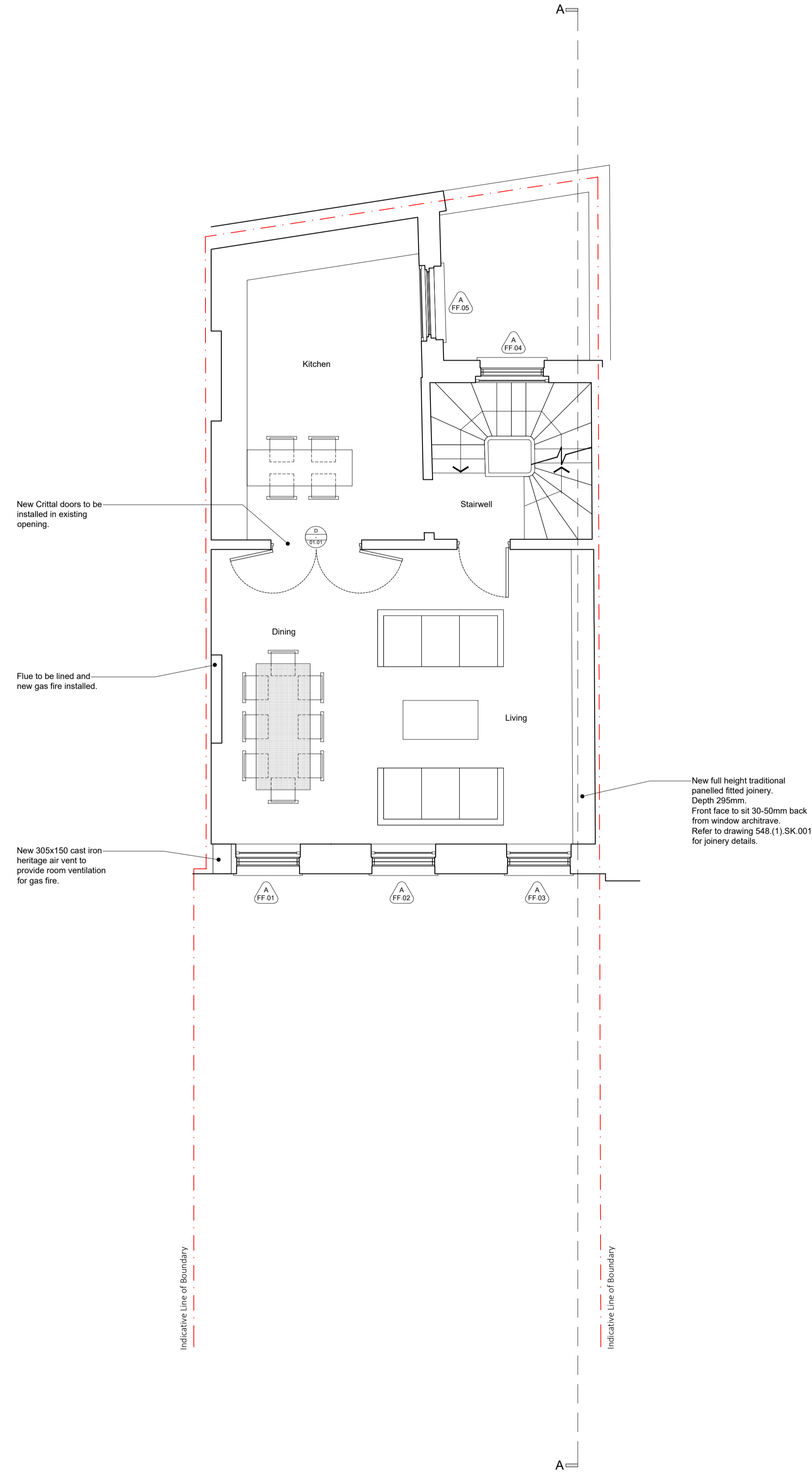
Proposed First Floor Plan
