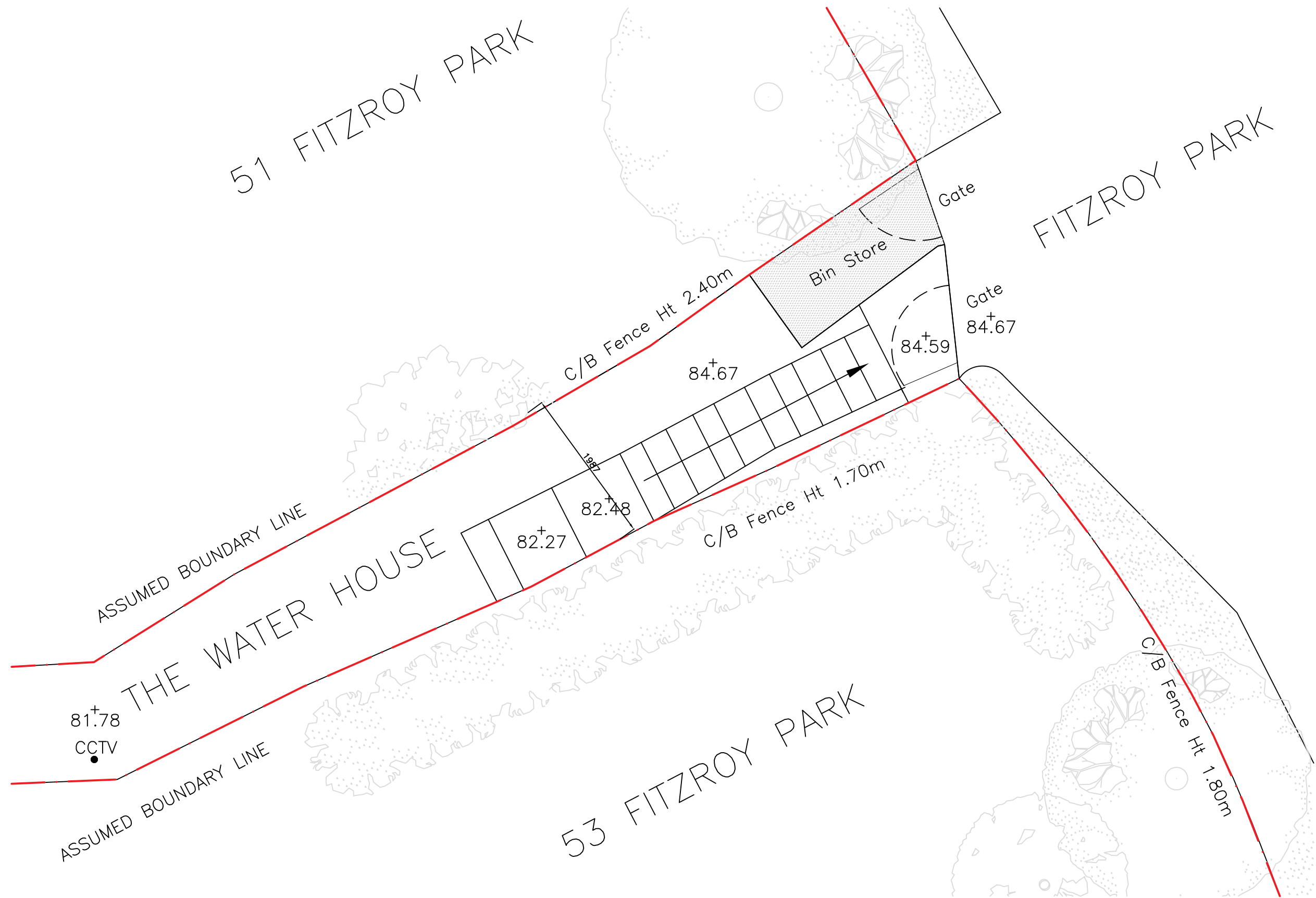
1 Existing Plan – External Platform Lift 1 : 25 @ A1
