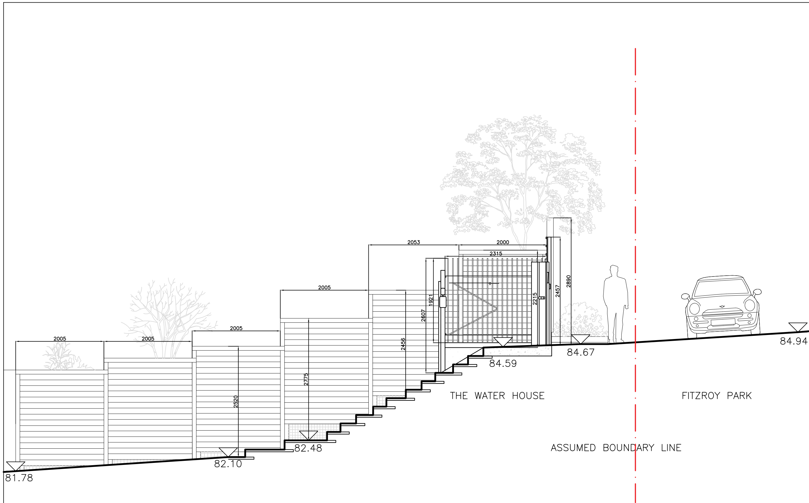
1 Existing Section - External Platform Lift 1:25 @ A1
