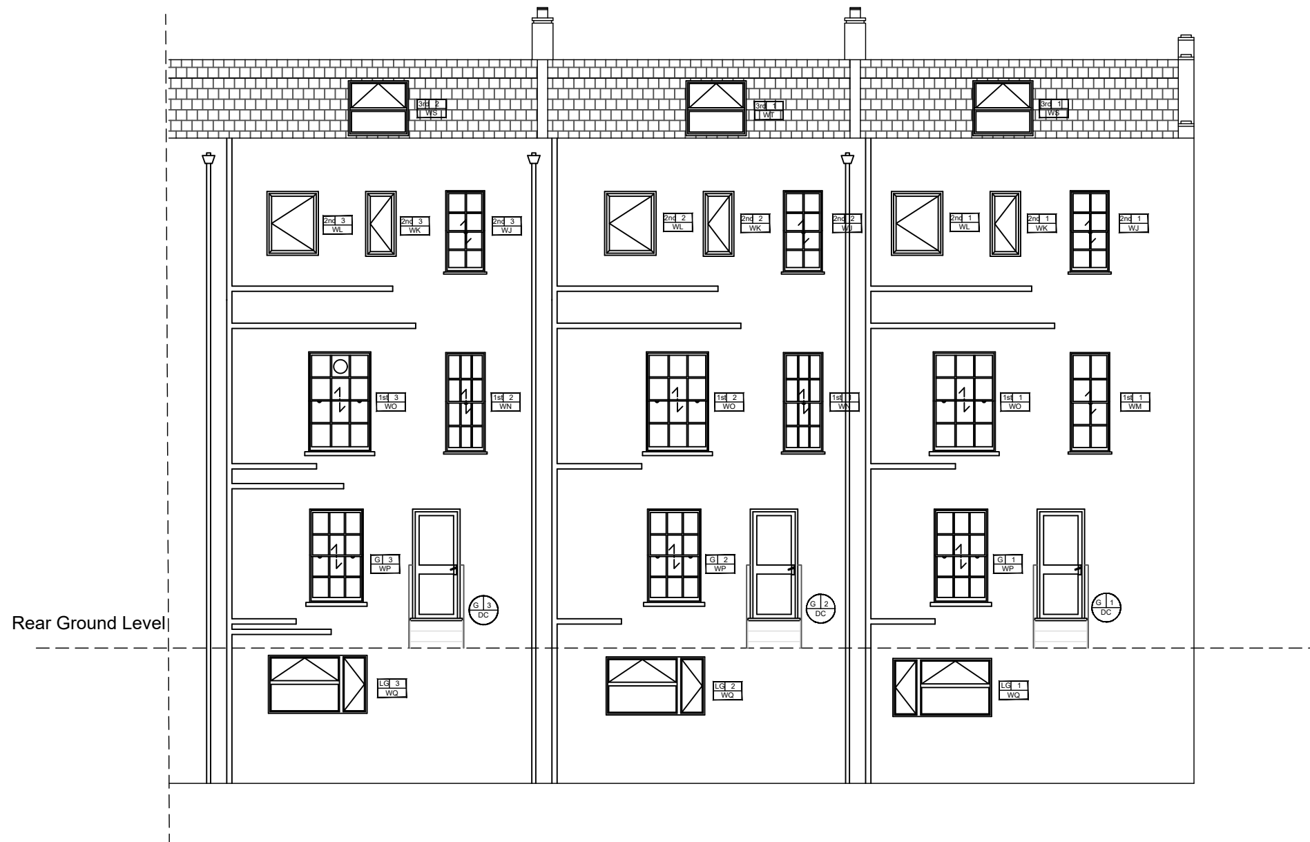
Rear Elevation
