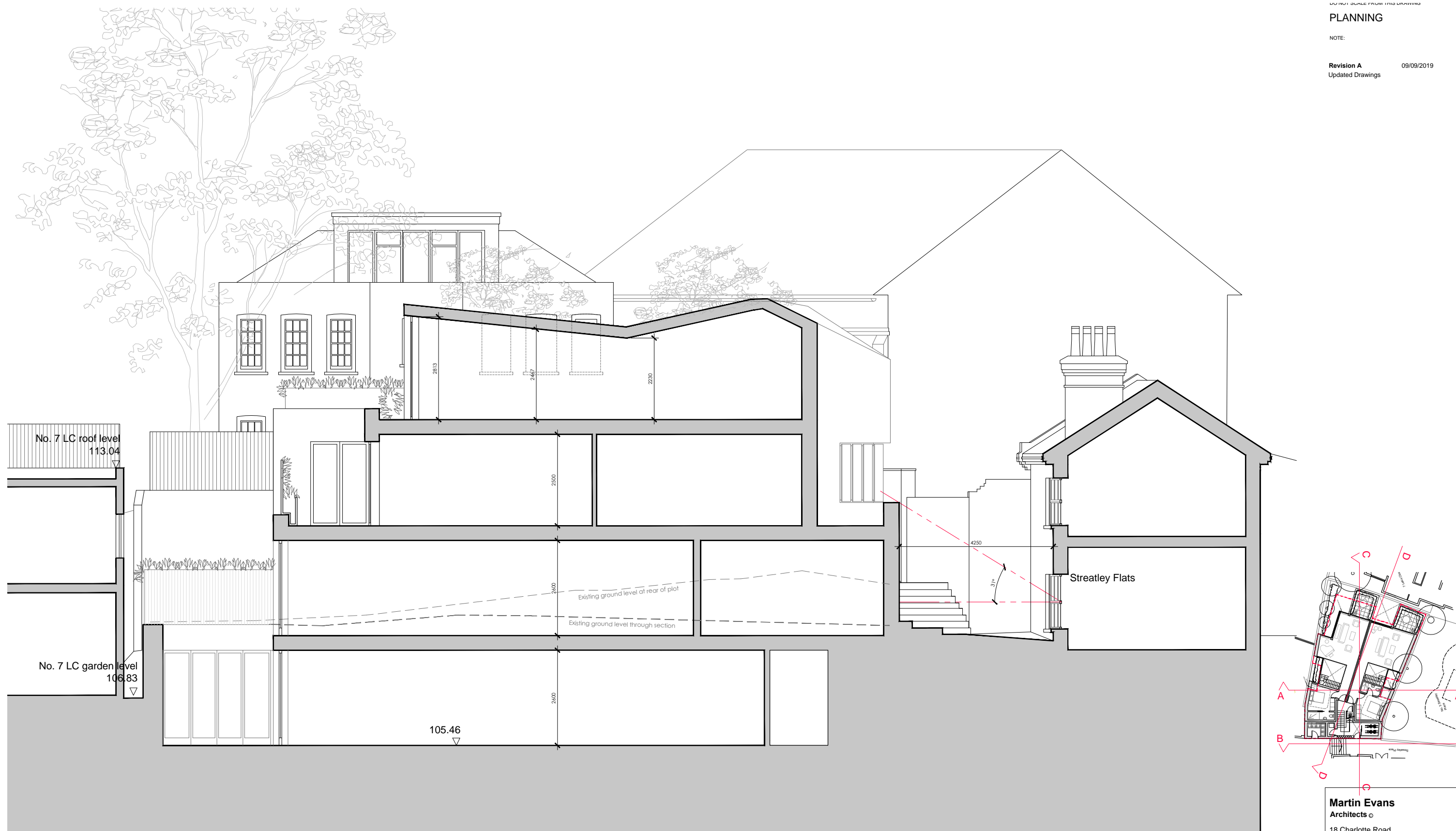
Proposed Section DD 1:100 @ A3 & 1:50 @ A1
