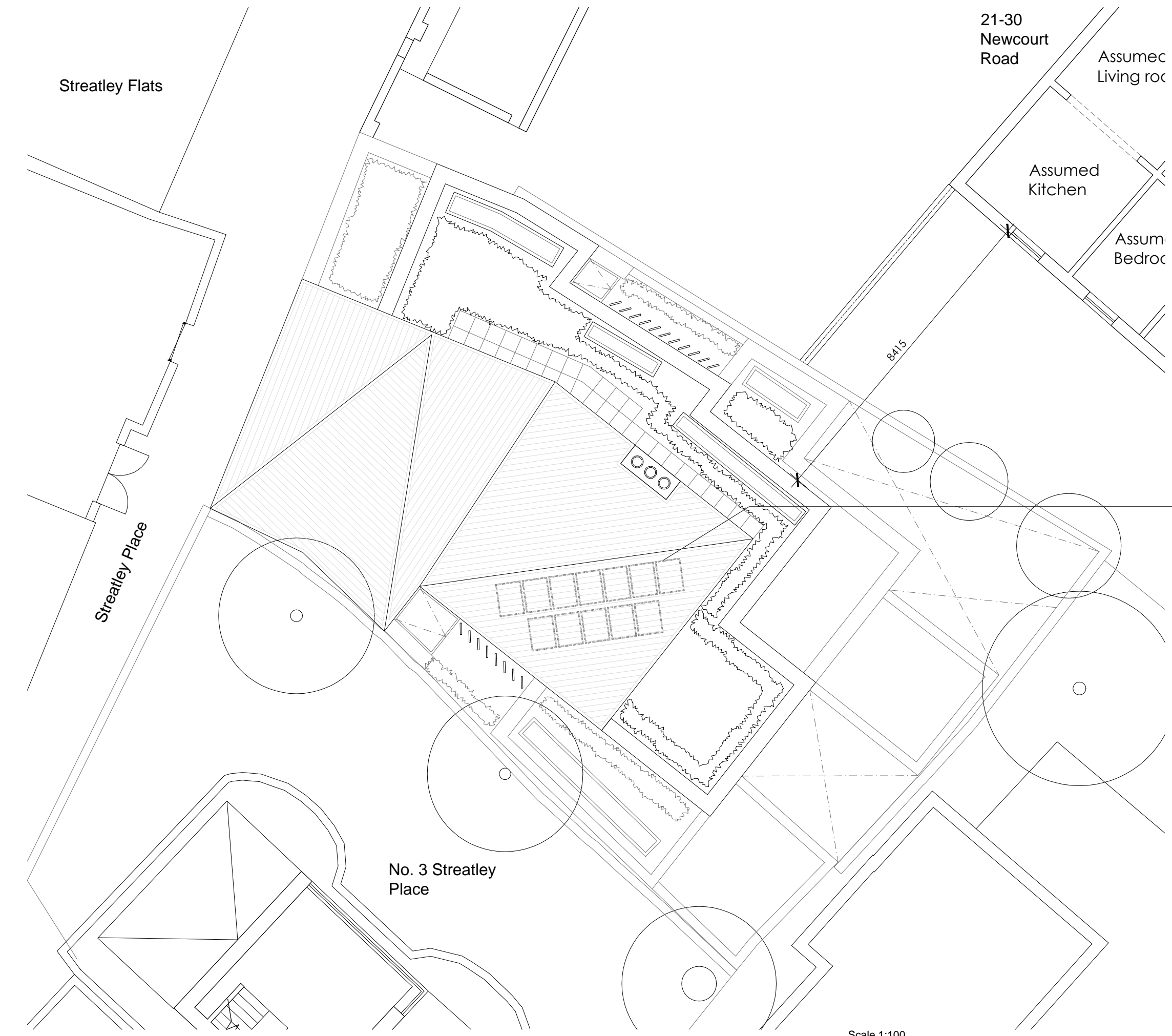
Proposed roof plan 1:100 @ A3 & 1:50 @ A1
