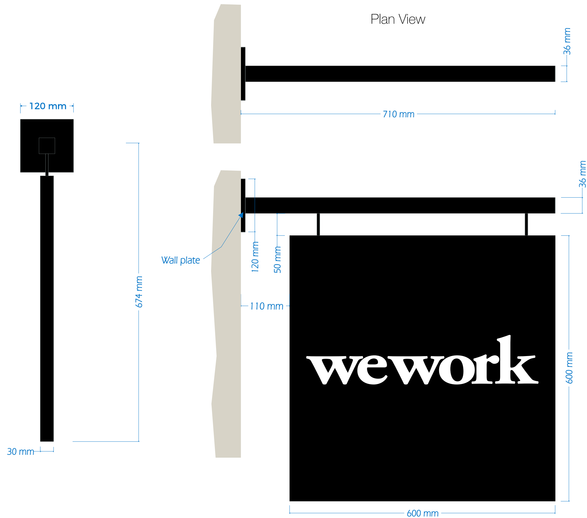
Sign P3 - Double sided 2mm Fabricated aluminium non-illuminated projection hanging sign with vinyl graphics to face
