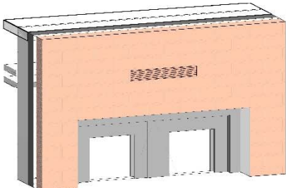
3D study of the façade for Flat type A6.08.02 illustrating MVHR intake and extract ventilation grilles
