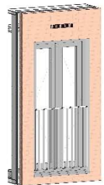
3D study of the façade for Flat type A6.08.02 illustrating MVHR intake and extract ventilation grilles
