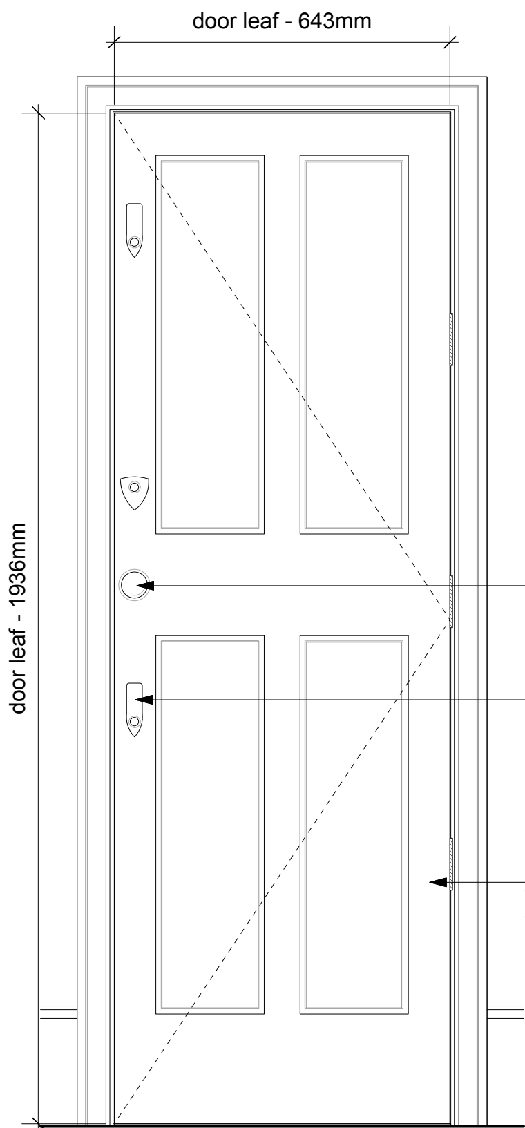
1 503 Landing Door Elevation Scale: 1:10
