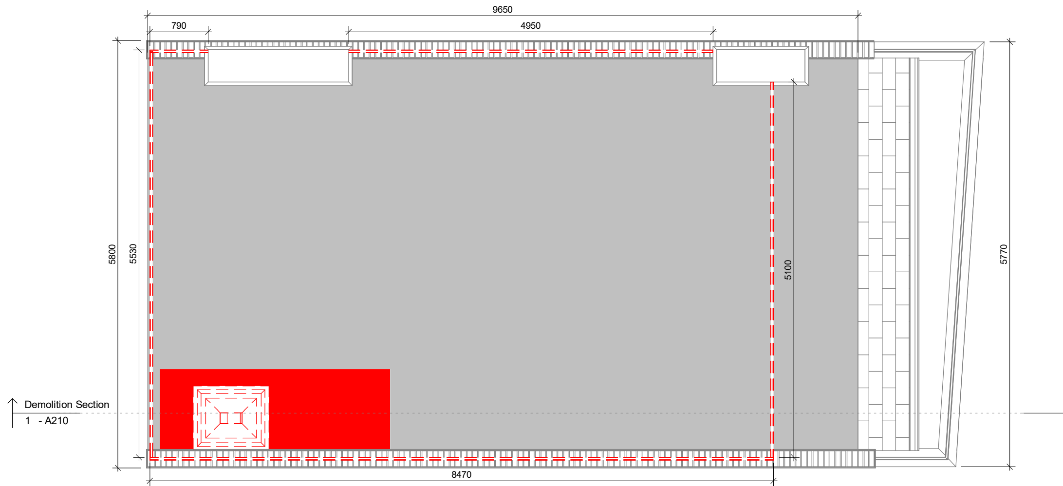
1 Demolition Roof 1 : 50
