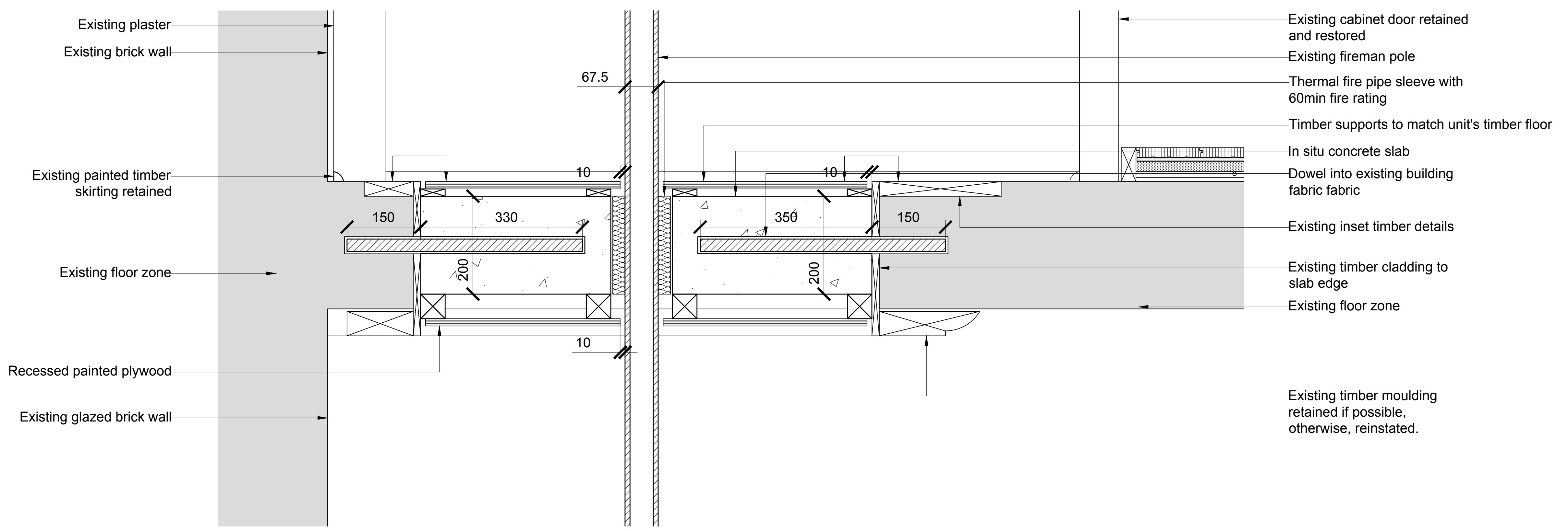
2 - Fireman Pole Cabinet 1:20 Plan Diagram
