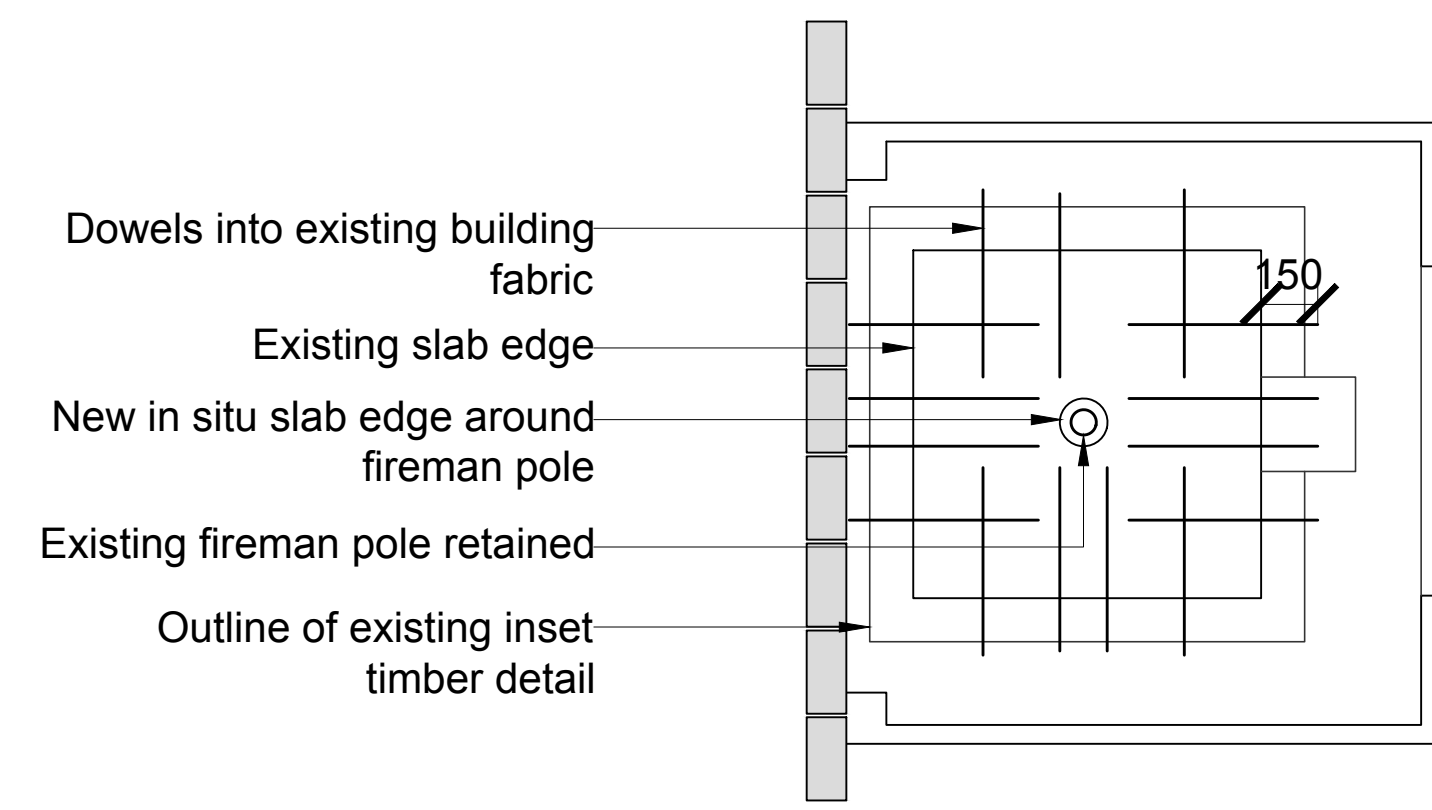
2 - Fireman Pole Cabinet 1:20 Plan Diagram
