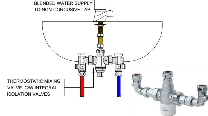
WASH HAND BASINS THERMOSTATIC MIXING VALVE ARRANGEMENT
