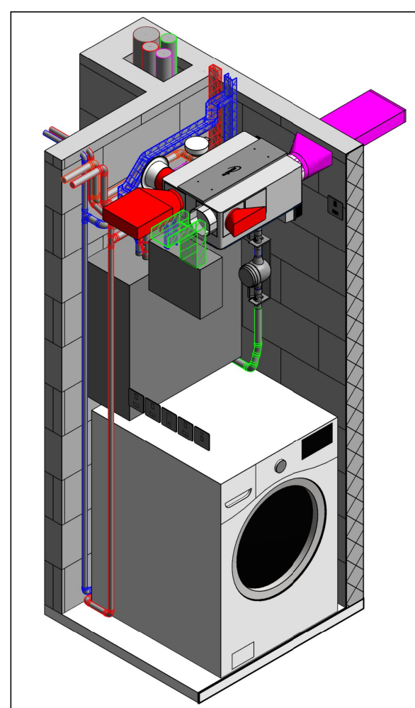
TYPICAL UTILITY ROOM DETAIL N.T.S. ILLUSTRATING WALL MOUNTED HEAT INTERFACE UNIT, CWS METER AND ASSOCIATED VALVES AND PIPEWORK. DETAILED COORDINATION BY CONTRACTOR.
