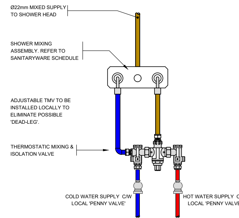
DETAIL M13.02 - SHOWER THERMOSTATIC MIXING VALVE ARRANGEMENT
