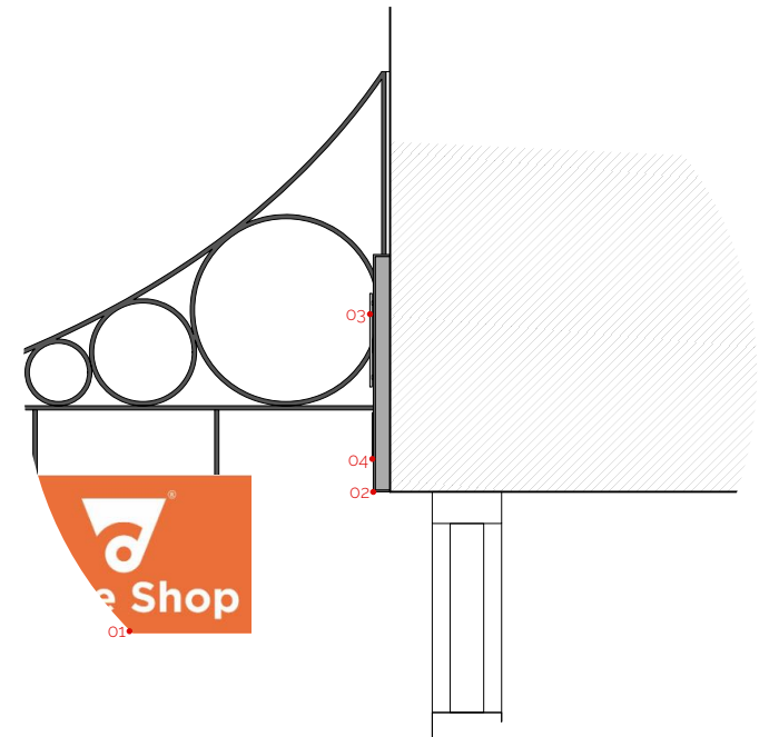
DETAIL AA @ 1/20
