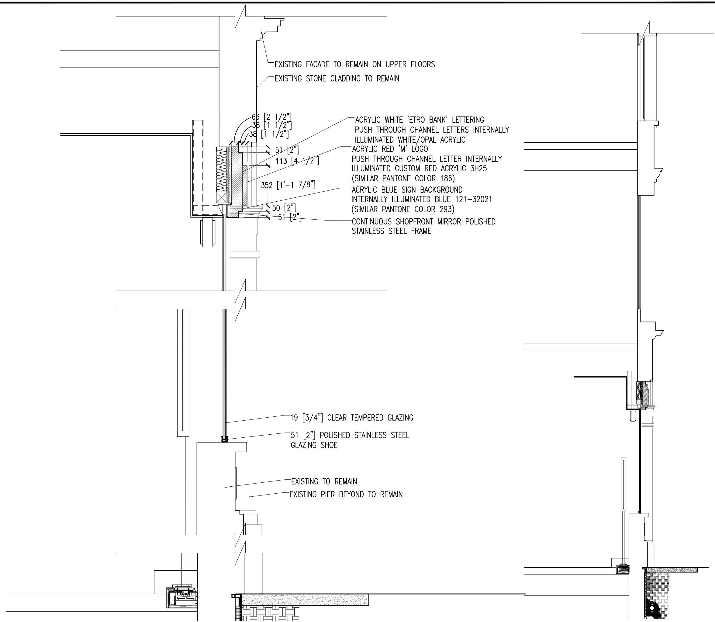
① OVERALL PROPOSED GLAZING & SIGNAGE
