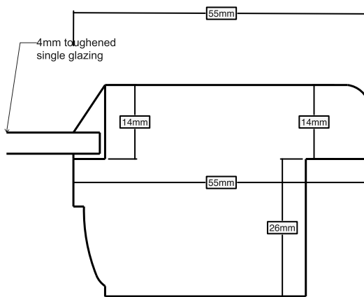
Section E-E
