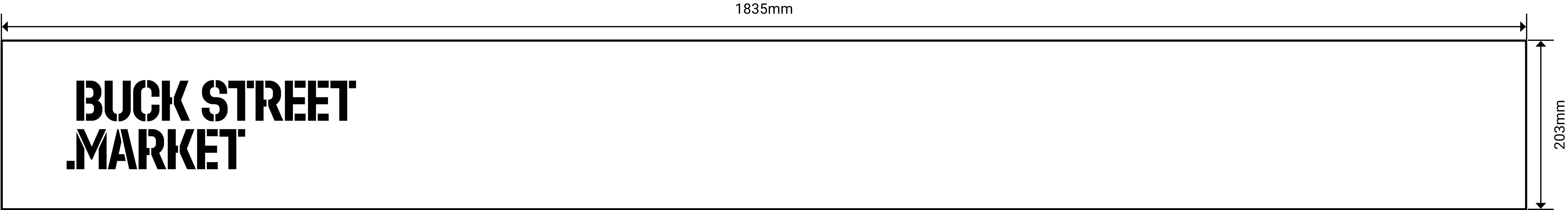
Façade Plate Painted Metal Stencil Cut Lettering Front-Facing View
