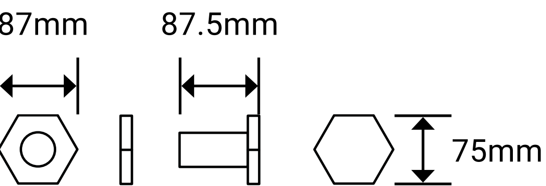
Fixing Washer and Bolt to Façade Plate Painted Metal
