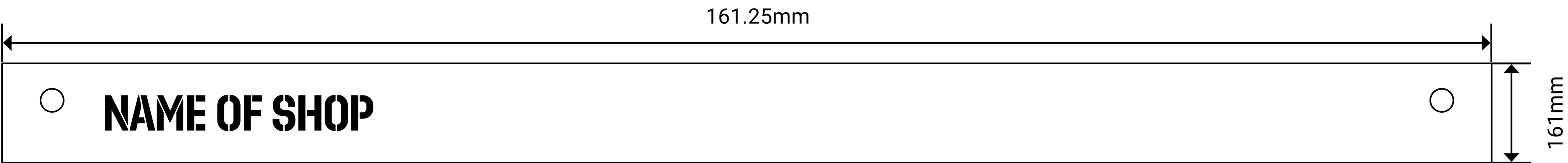
Façade Plate Painted Metal Adhesive Cut Vinyl Lettering Front-Facing View
