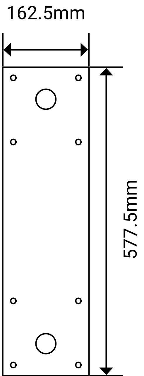
Projecting Sign Base Plate Painted Metal Front-Facing View
