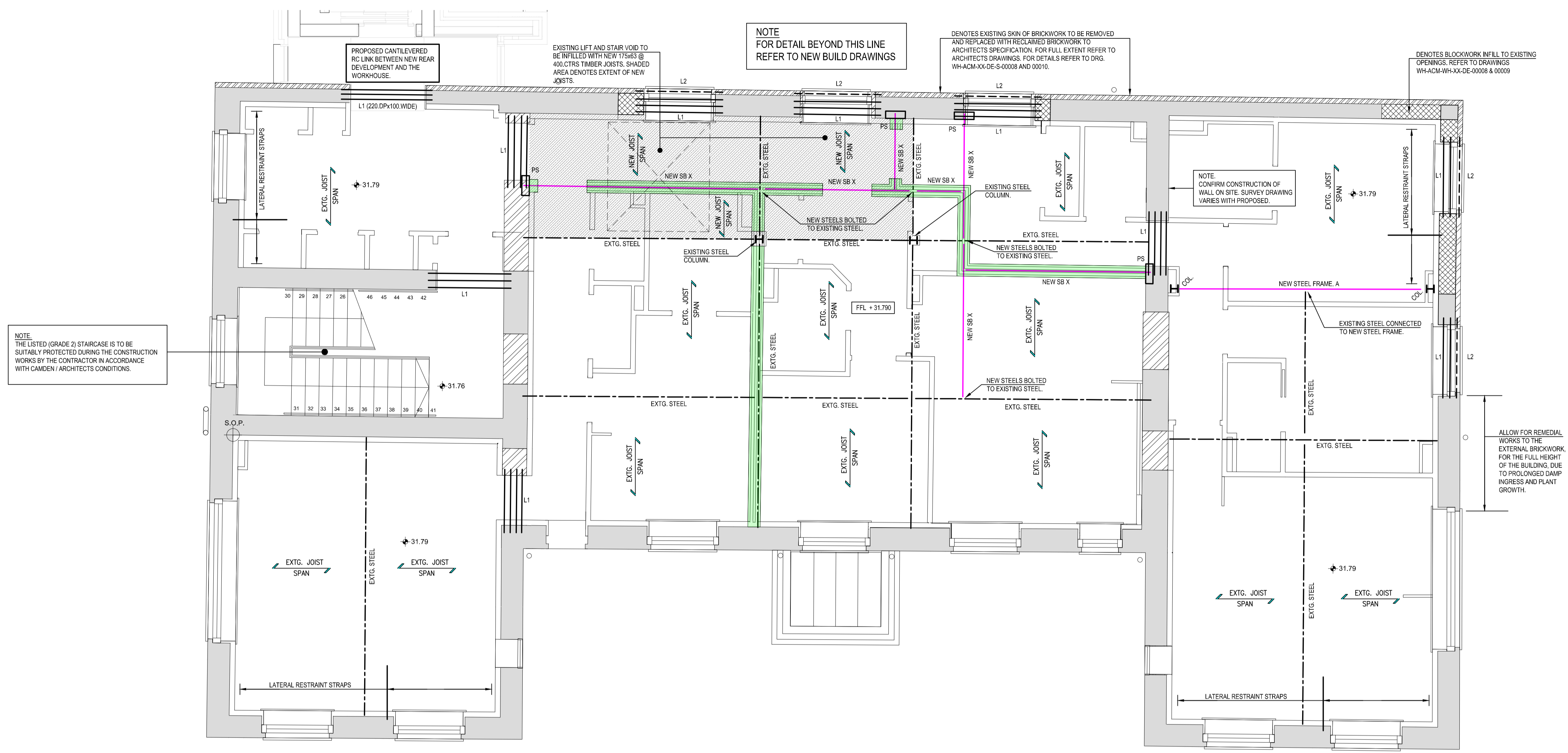
PROPOSED FIRST FLOOR PLAN [ LEVEL 01 ] 1:50 @ A1
