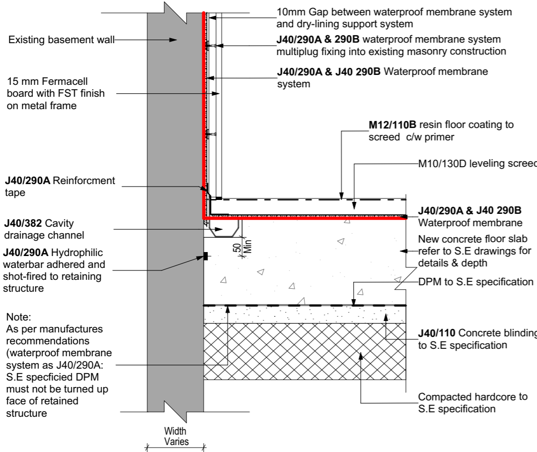
D01 TYPICAL BASEMENT EDGE DETAIL 1:10
