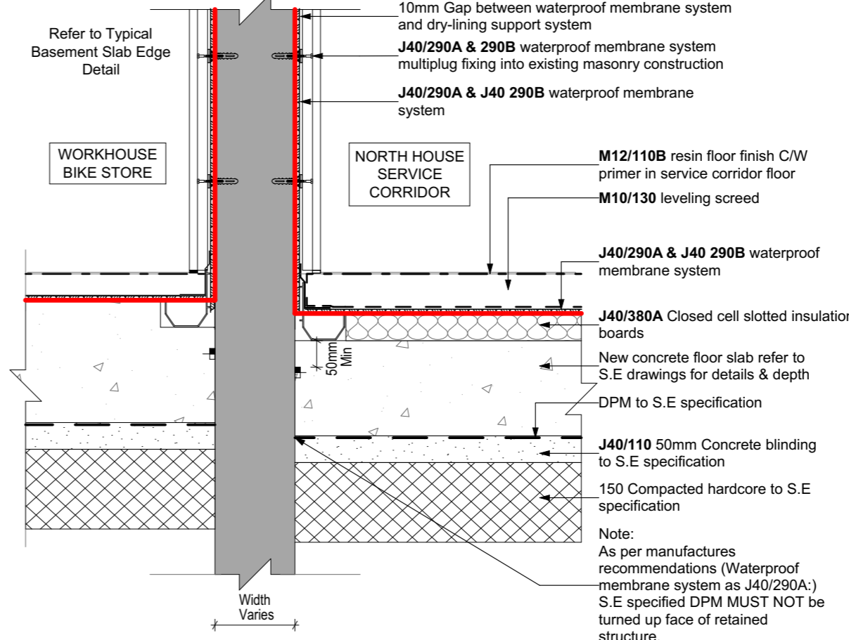
D02 BASEMENT RETAINED WALL INTERFACE W/ NEW SLAB 1:10
