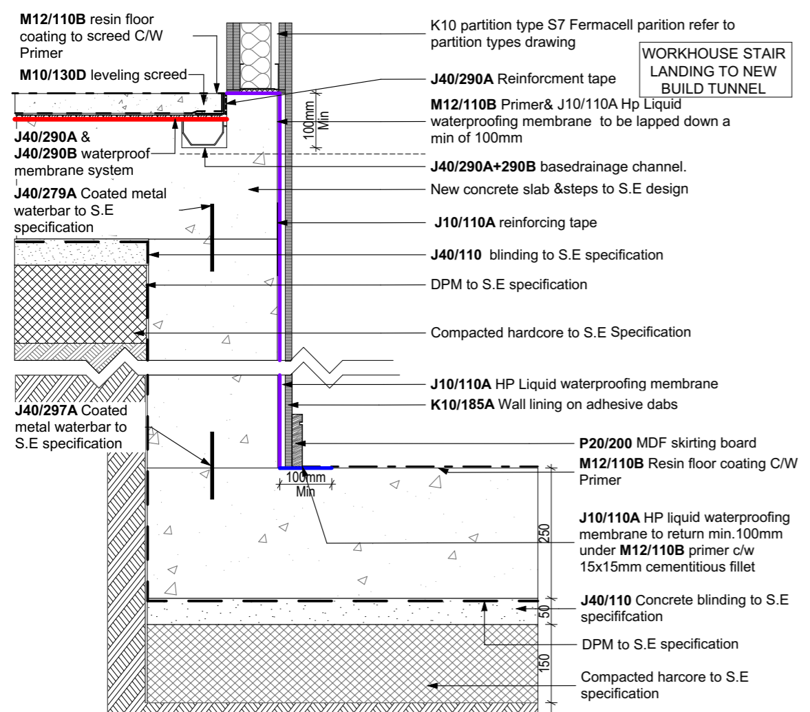
D03 BASEMENT LEVEL CHANGE DETAIL 1:10
