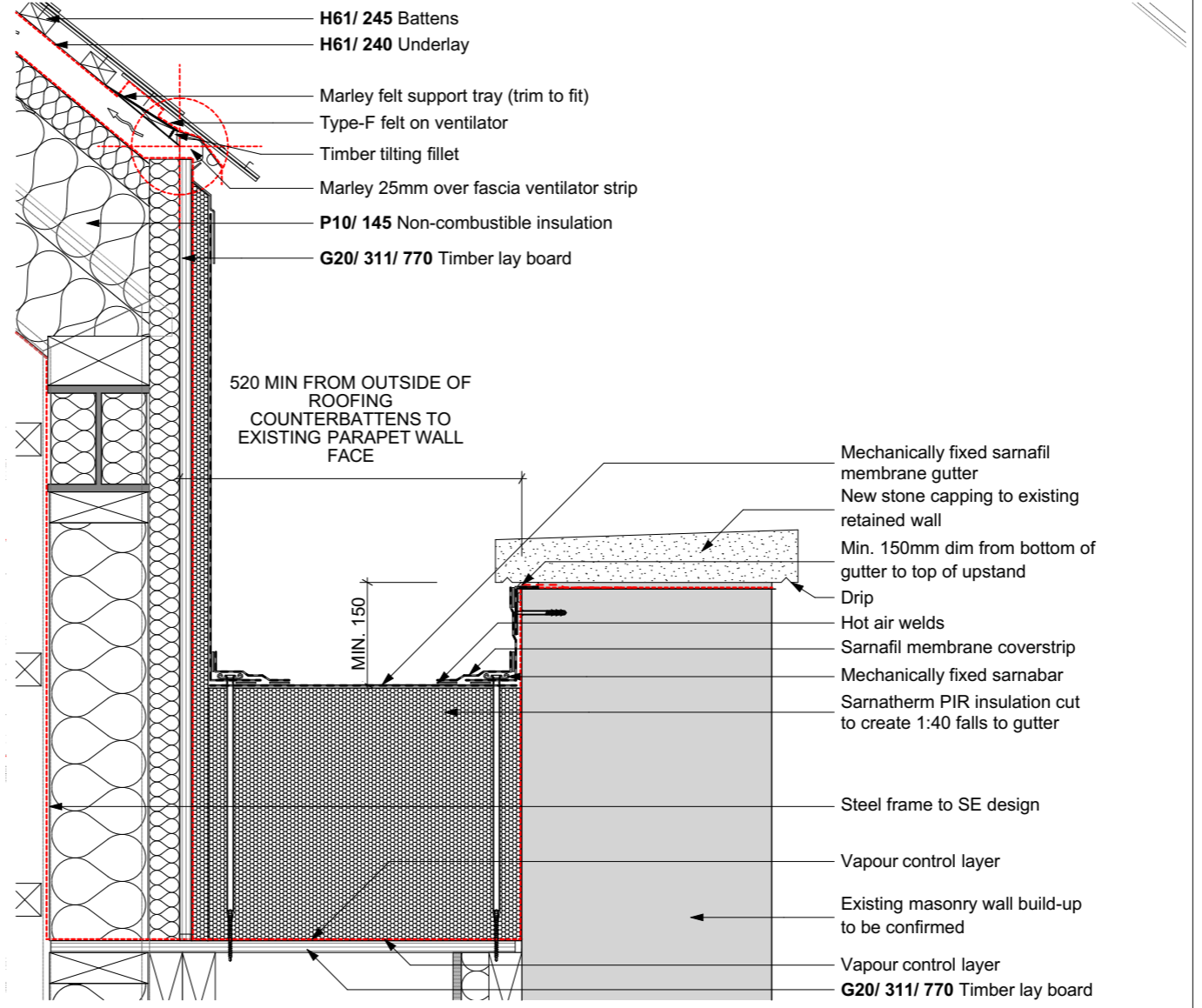
D05 GUTTER DETAIL 1:10
