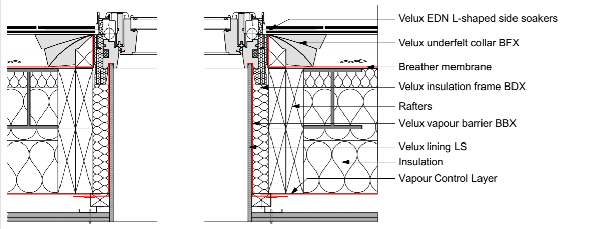
D02 ROOF WINDOW JAMB 1:10
