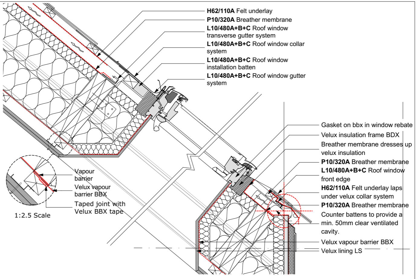
D04 ROOF WINDOW HEAD AND SILL 1:10
