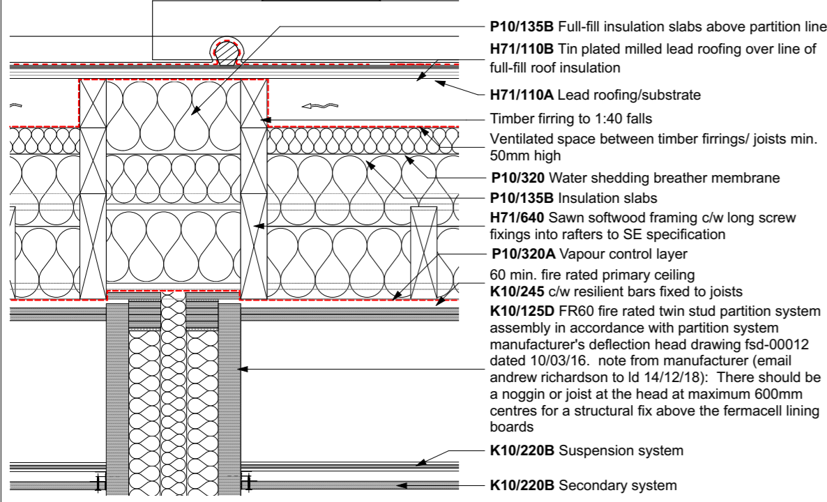
D03 FIRE STOPPING TO PARTY WALL ROOF JUNCTION 1:10
