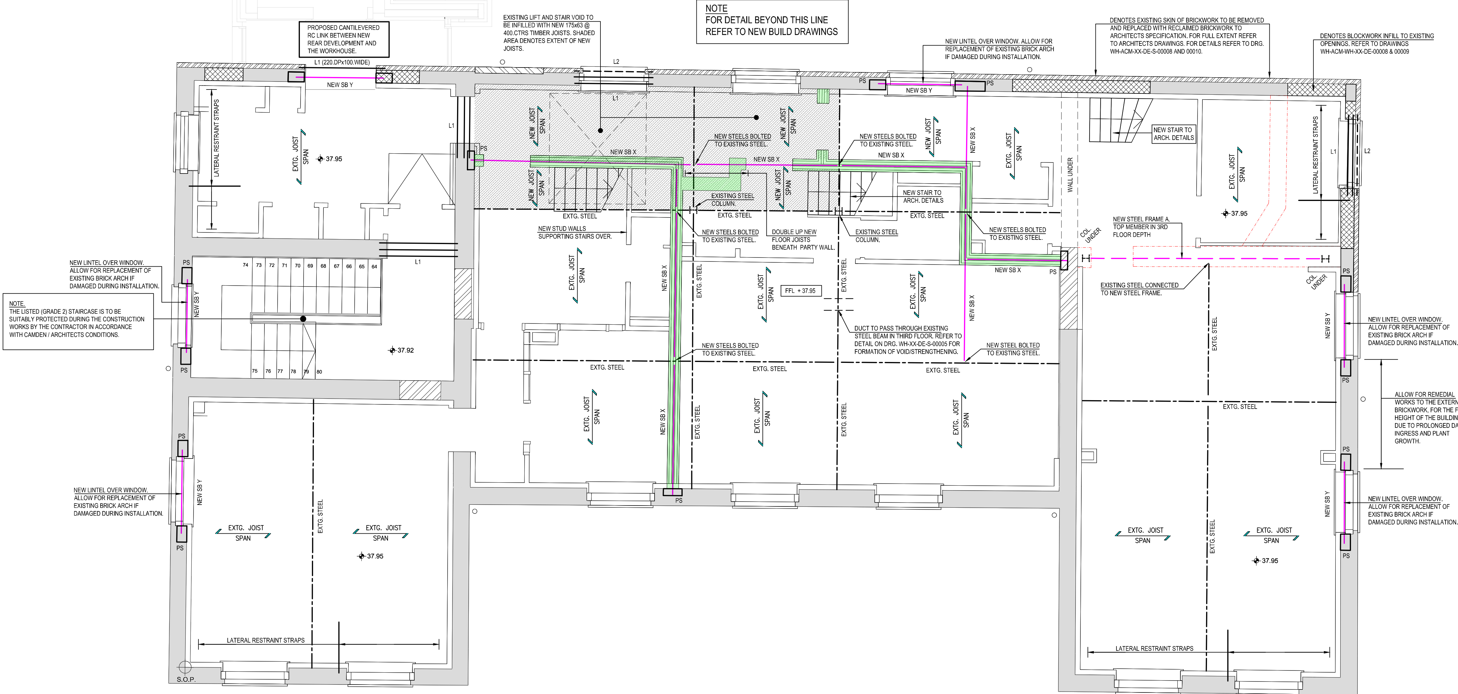
PROPOSED THIRD FLOOR PLAN [ LEVEL 03 ]
