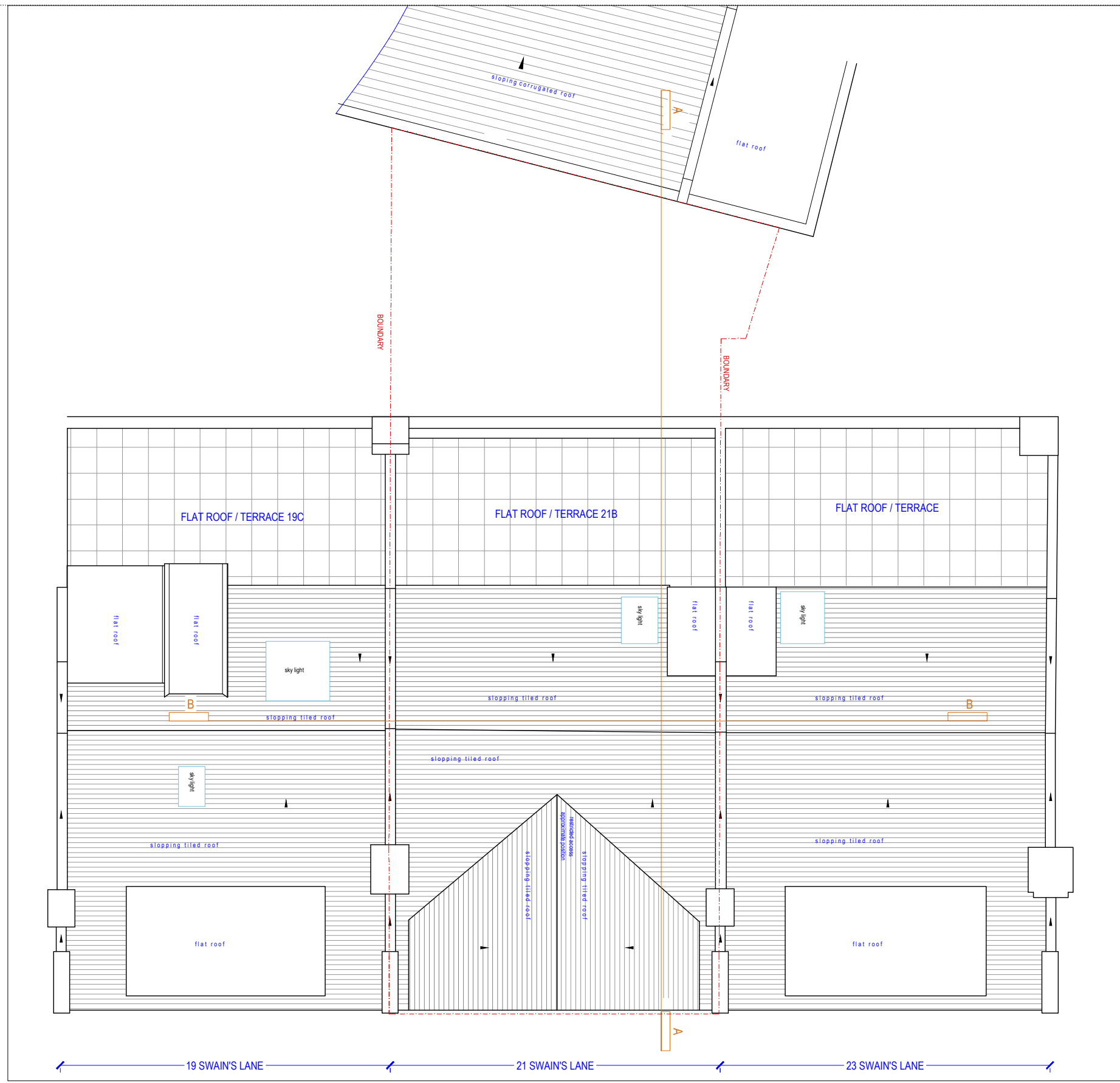
[01] EXISTING ROOF PLAN @1:100
