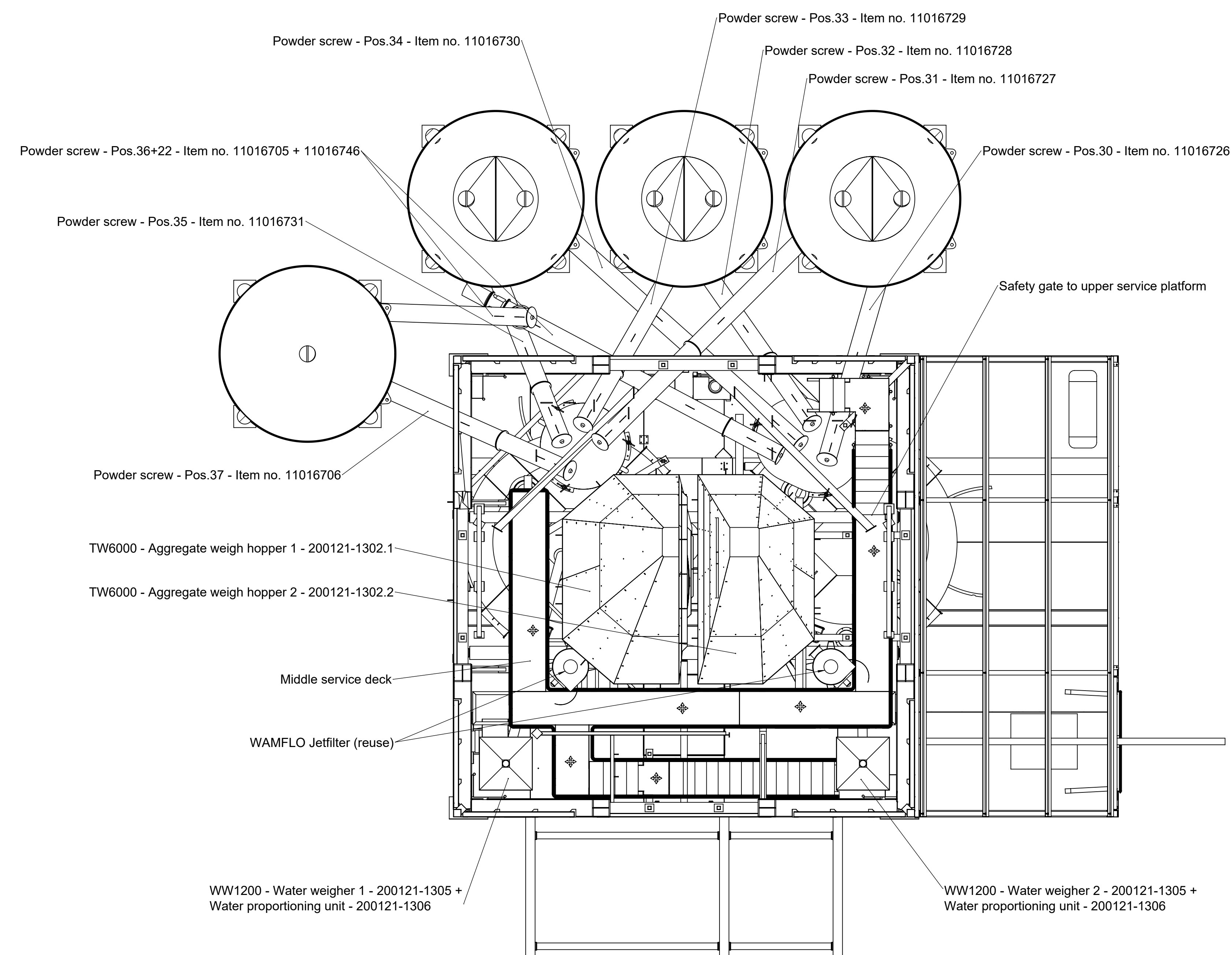
SECTION C-C
