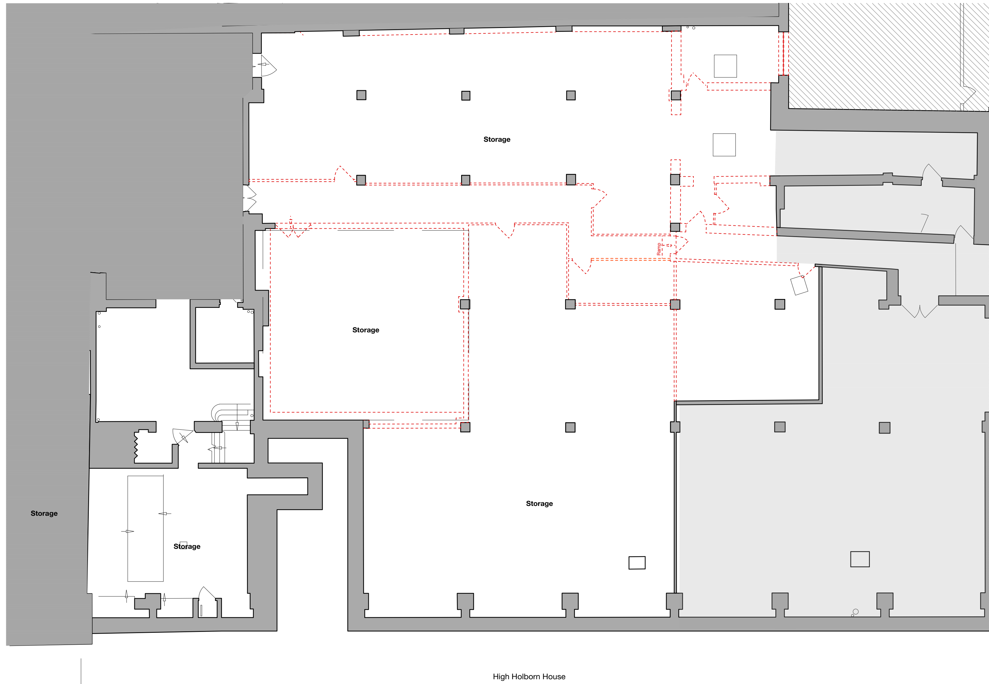
1 High Holborn House Demolition Basement Scale: 1:100
