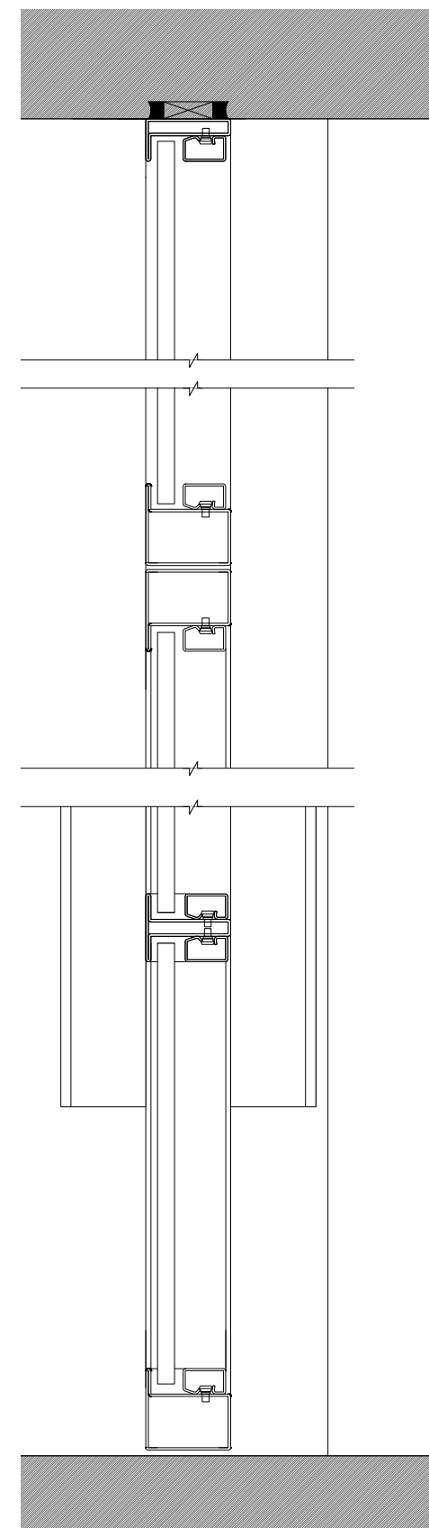
Head detail 1:2
